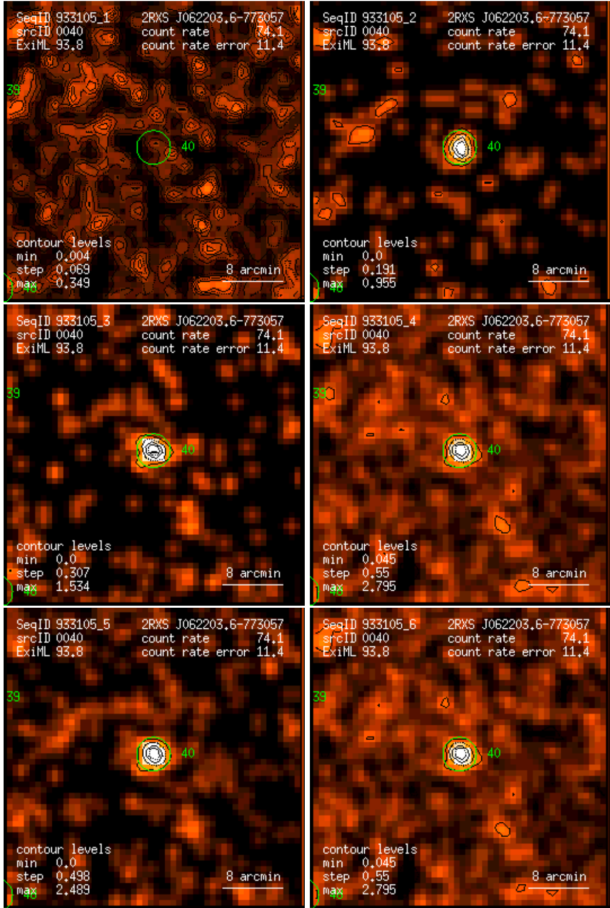
Figure 40: RASS 933105: detection 0040: band rate images, Gaussian filter: (1) PSPC channels 11 – 41, (2) 52 – 90, (3) 91 – 201, (4) 11 – 235, (5) 52 – 201, (6) 11 – 201. Broad band rates in counts/ks. Band rate contour levels in counts/ks/arcmin 2 .
