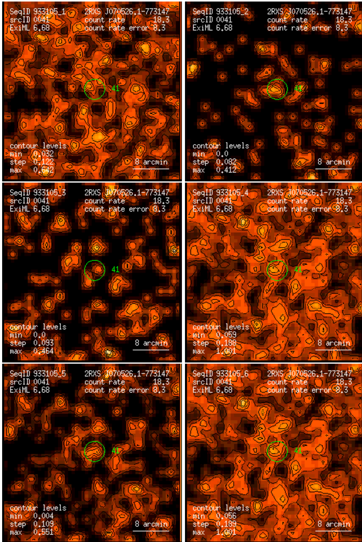
Figure 41: RASS 933105: detection 0041: band rate images, Gaussian filter: (1) PSPC channels 11 – 41, (2) 52 – 90, (3) 91 – 201, (4) 11 – 235, (5) 52 – 201, (6) 11 – 201. Broad band rates in counts/ks. Band rate contour levels in counts/ks/arcmin 2 .
