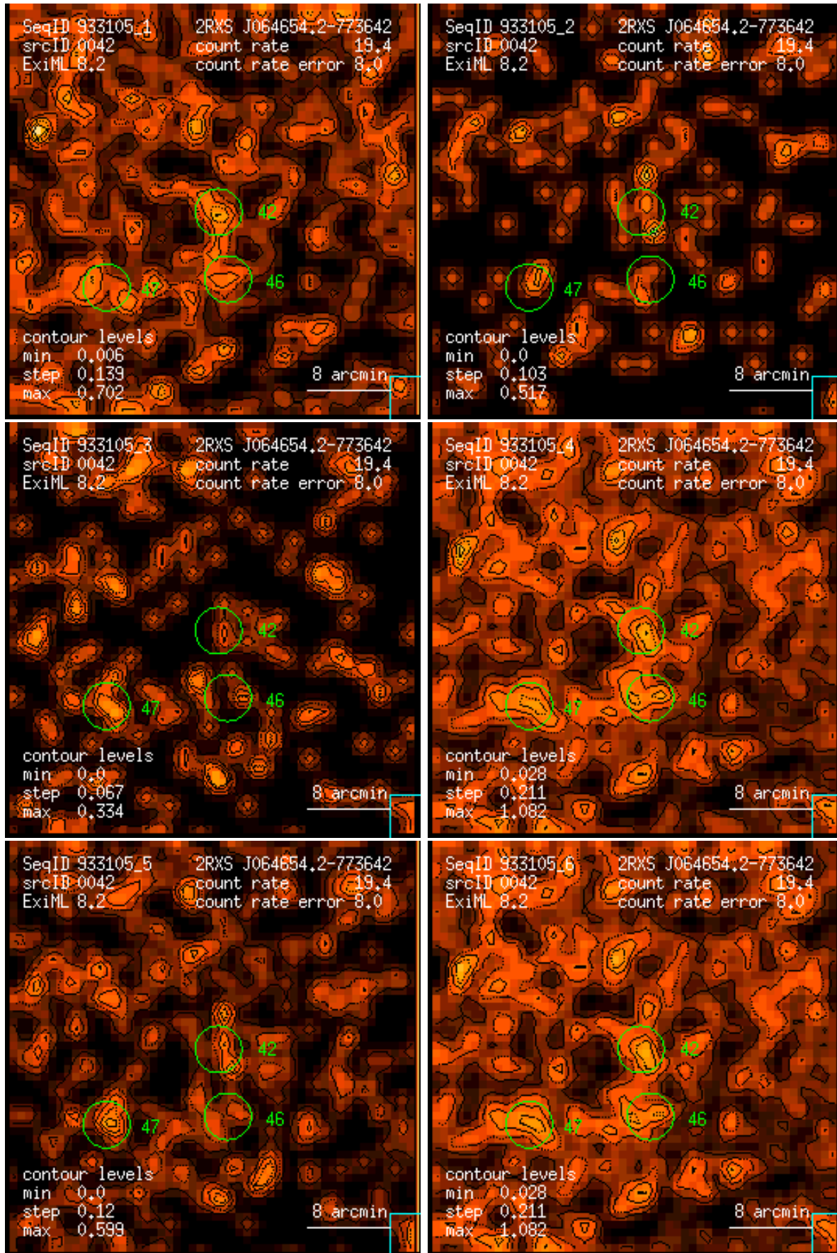
Figure 42: RASS 933105: detection 0042: band rate images, Gaussian filter: (1) PSPC channels 11 – 41, (2) 52 – 90, (3) 91 – 201, (4) 11 – 235, (5) 52 – 201, (6) 11 – 201. Broad band rates in counts/ks. Band rate contour levels in counts/ks/arcmin 2 .
