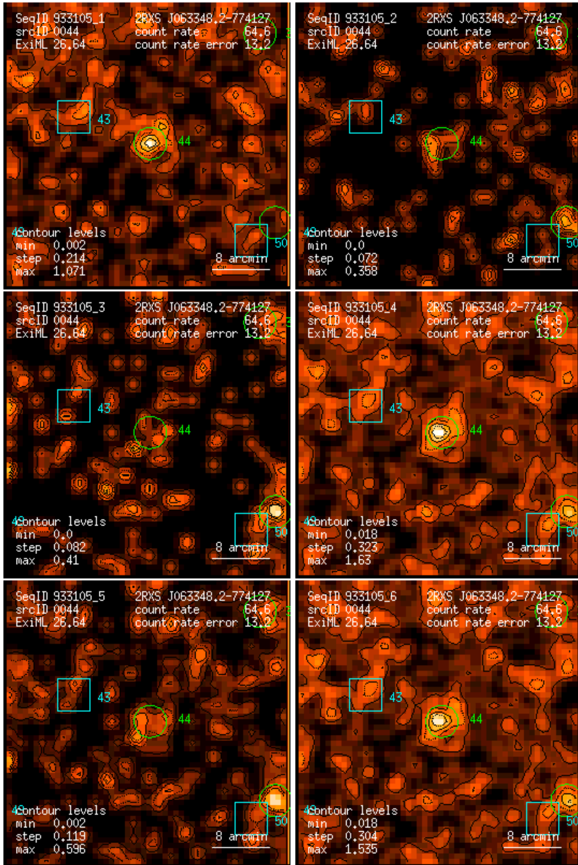
Figure 44: RASS 933105: detection 0044: band rate images, Gaussian filter: (1) PSPC channels 11 – 41, (2) 52 – 90, (3) 91 – 201, (4) 11 – 235, (5) 52 – 201, (6) 11 – 201. Broad band rates in counts/ks. Band rate contour levels in counts/ks/arcmin 2 .
