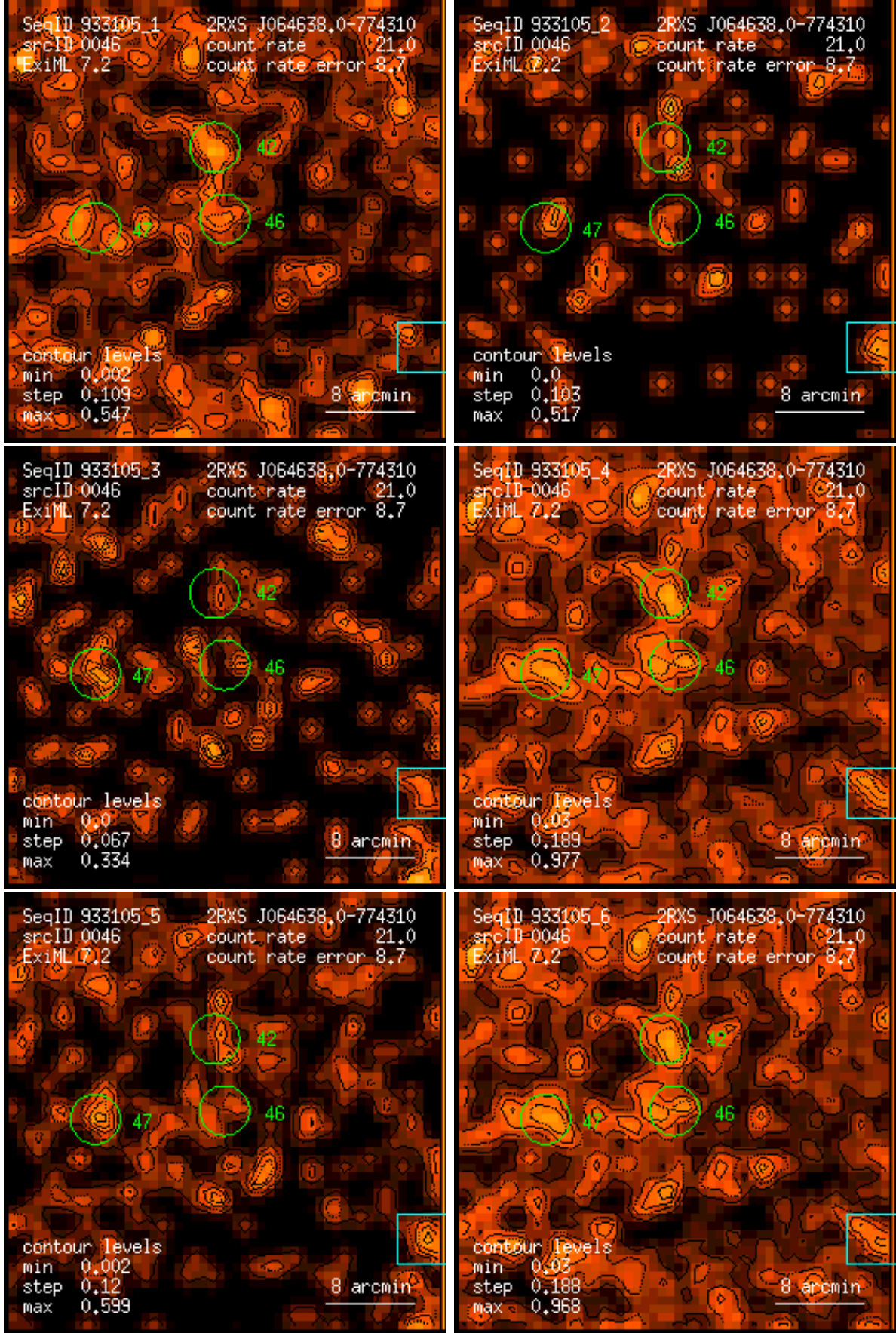
Figure 46: RASS 933105: detection 0046: band rate images, Gaussian filter: (1) PSPC channels 11 – 41, (2) 52 – 90, (3) 91 – 201, (4) 11 – 235, (5) 52 – 201, (6) 11 – 201. Broad band rates in counts/ks. Band rate contour levels in counts/ks/arcmin 2 .
