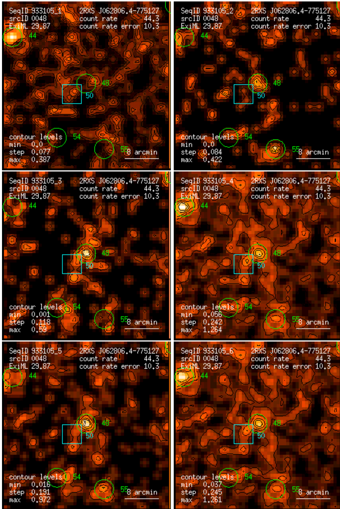
Figure 48: RASS 933105: detection 0048: band rate images, Gaussian filter: (1) PSPC channels 11 – 41, (2) 52 – 90, (3) 91 – 201, (4) 11 – 235, (5) 52 – 201, (6) 11 – 201. Broad band rates in counts/ks. Band rate contour levels in counts/ks/arcmin 2 .
