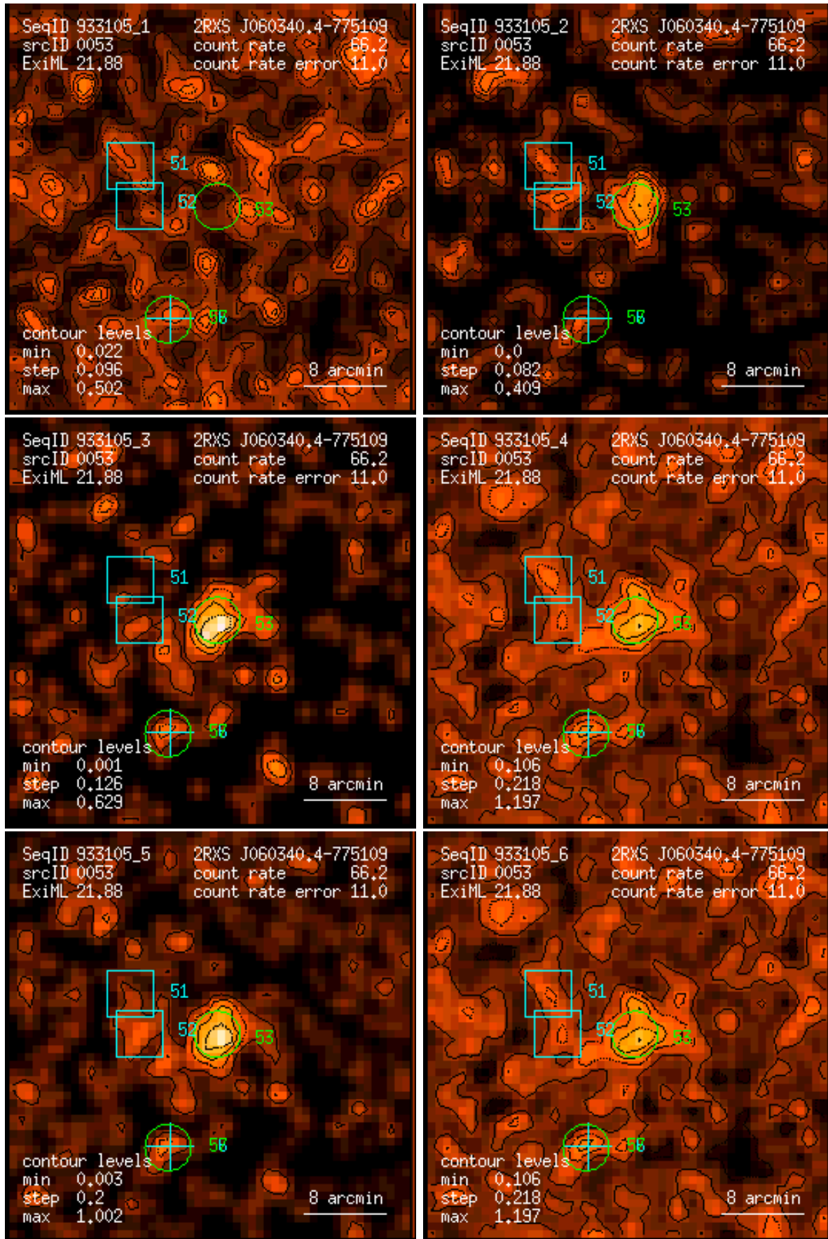
Figure 53: RASS 933105: detection 0053: band rate images, Gaussian filter: (1) PSPC channels 11 – 41, (2) 52 – 90, (3) 91 – 201, (4) 11 – 235, (5) 52 – 201, (6) 11 – 201. Broad band rates in counts/ks. Band rate contour levels in counts/ks/arcmin 2 .
