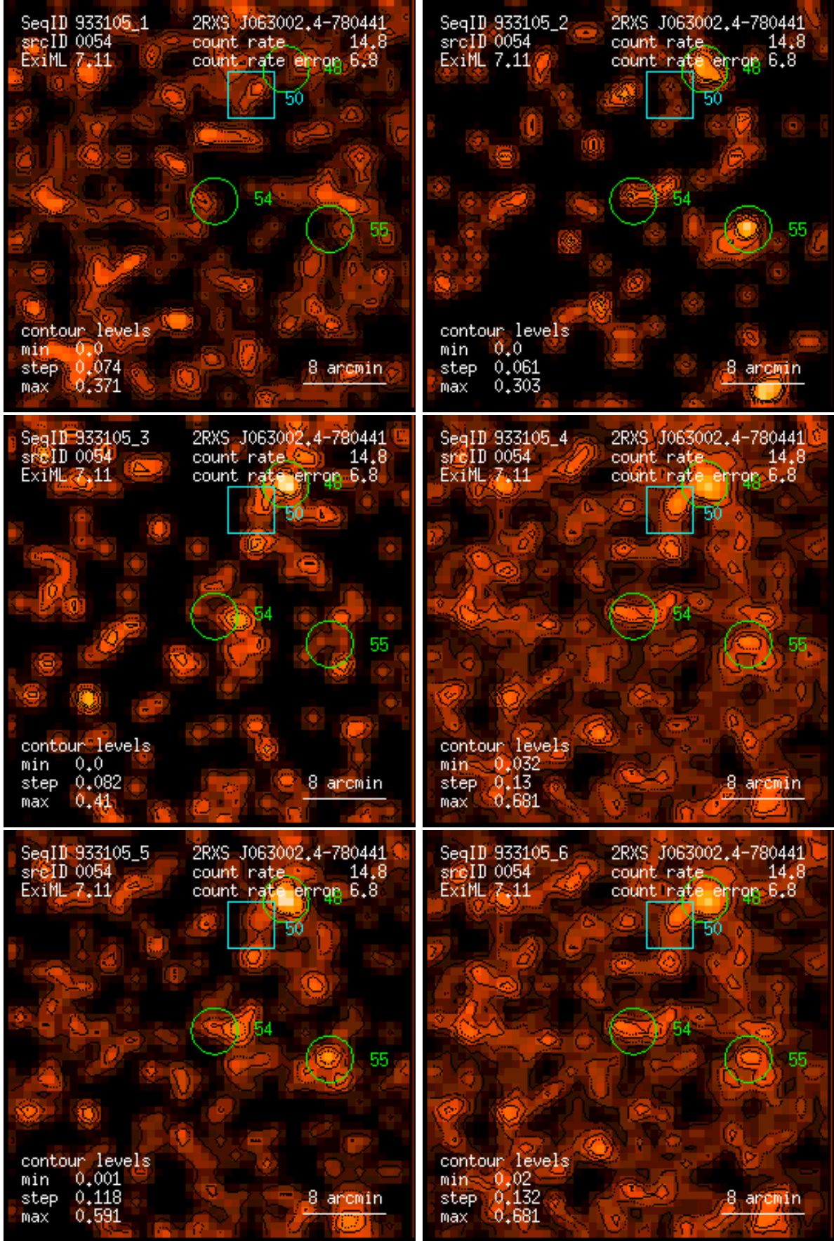
Figure 54: RASS 933105: detection 0054: band rate images, Gaussian filter: (1) PSPC channels 11 – 41, (2) 52 – 90, (3) 91 – 201, (4) 11 – 235, (5) 52 – 201, (6) 11 – 201. Broad band rates in counts/ks. Band rate contour levels in counts/ks/arcmin 2 .
