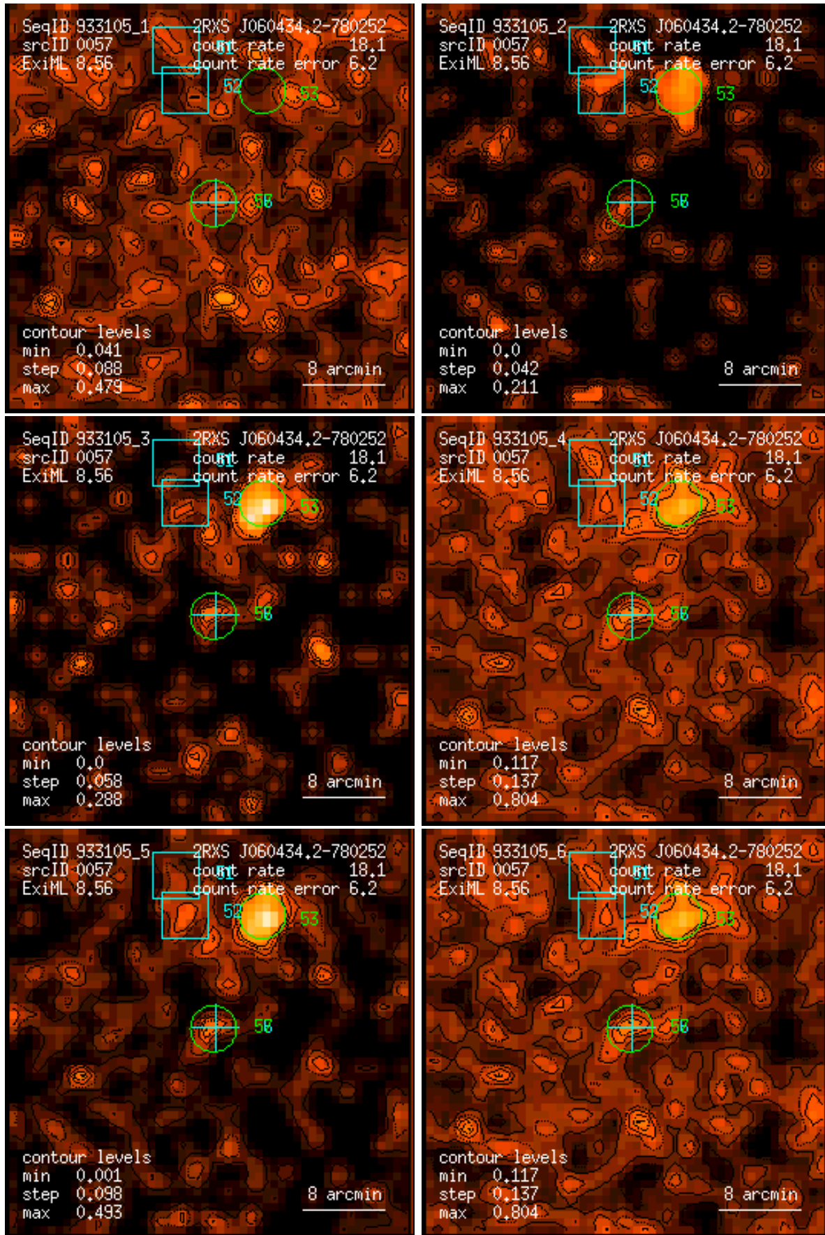
Figure 57: RASS 933105: detection 0057: band rate images, Gaussian filter: (1) PSPC channels 11 – 41, (2) 52 – 90, (3) 91 – 201, (4) 11 – 235, (5) 52 – 201, (6) 11 – 201. Broad band rates in counts/ks. Band rate contour levels in counts/ks/arcmin 2 .
