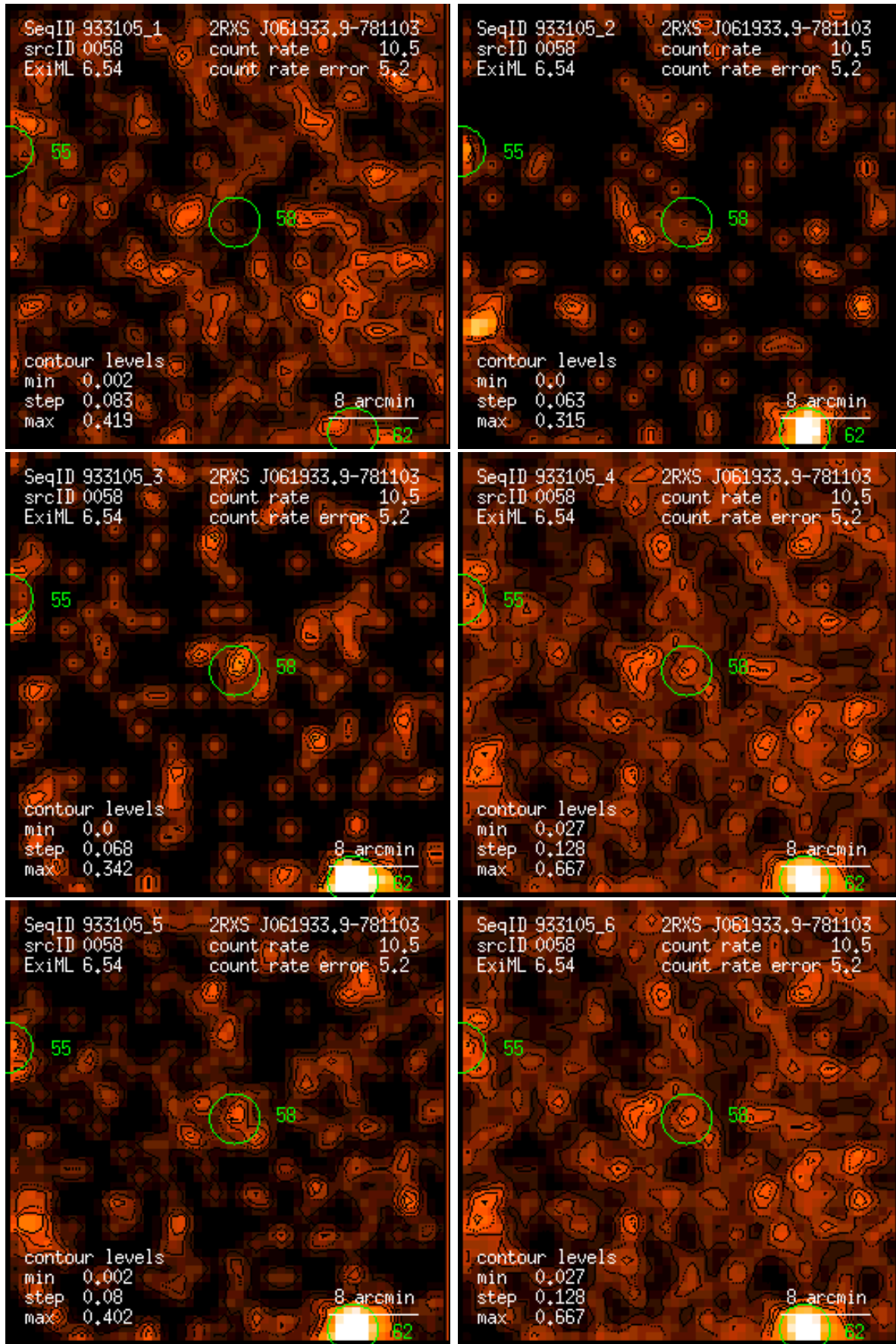
Figure 58: RASS 933105: detection 0058: band rate images, Gaussian filter: (1) PSPC channels 11 – 41, (2) 52 – 90, (3) 91 – 201, (4) 11 – 235, (5) 52 – 201, (6) 11 – 201. Broad band rates in counts/ks. Band rate contour levels in counts/ks/arcmin 2 .
