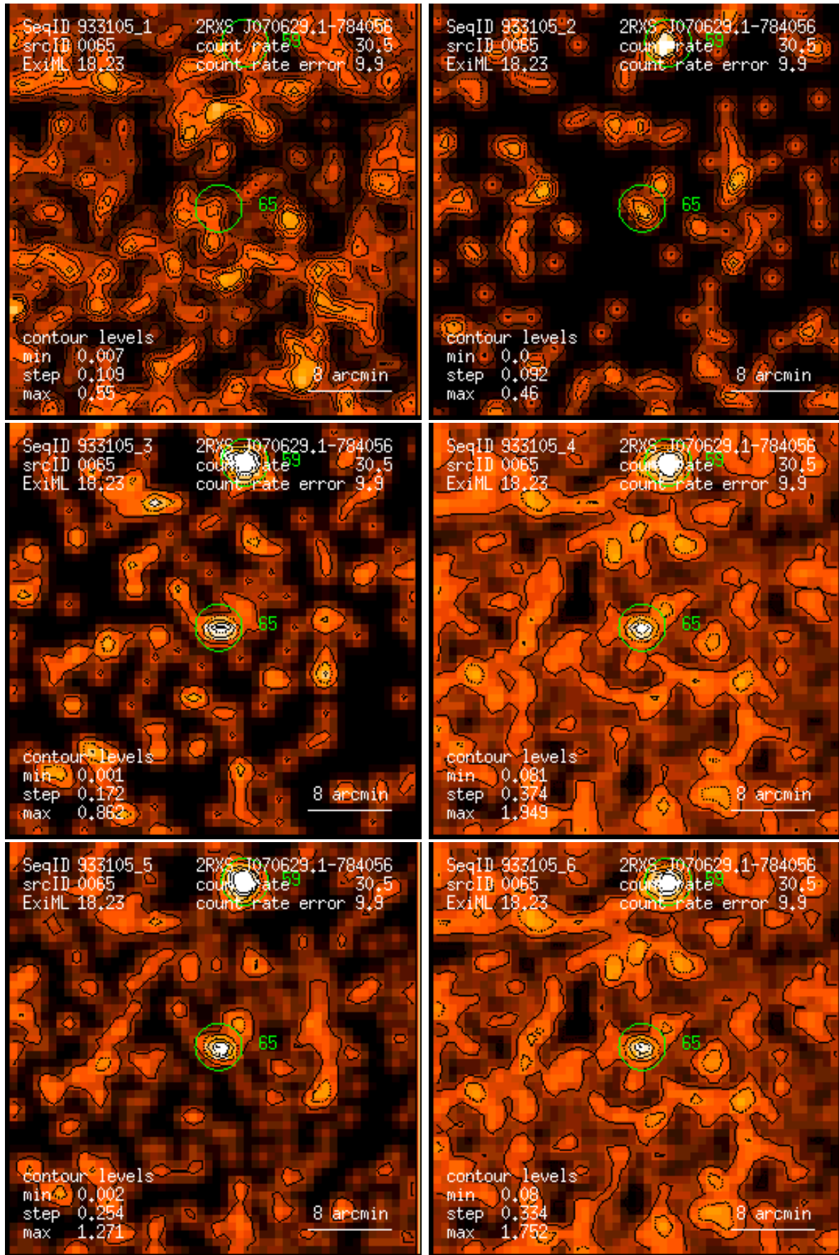
Figure 65: RASS 933105: detection 0065: band rate images, Gaussian filter: (1) PSPC channels 11 – 41, (2) 52 – 90, (3) 91 – 201, (4) 11 – 235, (5) 52 – 201, (6) 11 – 201. Broad band rates in counts/ks. Band rate contour levels in counts/ks/arcmin 2 .
