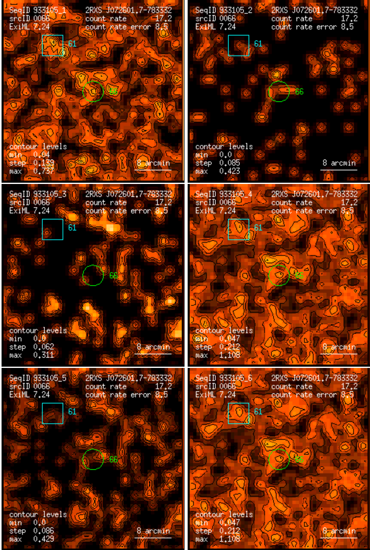
Figure 66: RASS 933105: detection 0066: band rate images, Gaussian filter: (1) PSPC channels 11 – 41, (2) 52 – 90, (3) 91 – 201, (4) 11 – 235, (5) 52 – 201, (6) 11 – 201. Broad band rates in counts/ks. Band rate contour levels in counts/ks/arcmin 2 .
