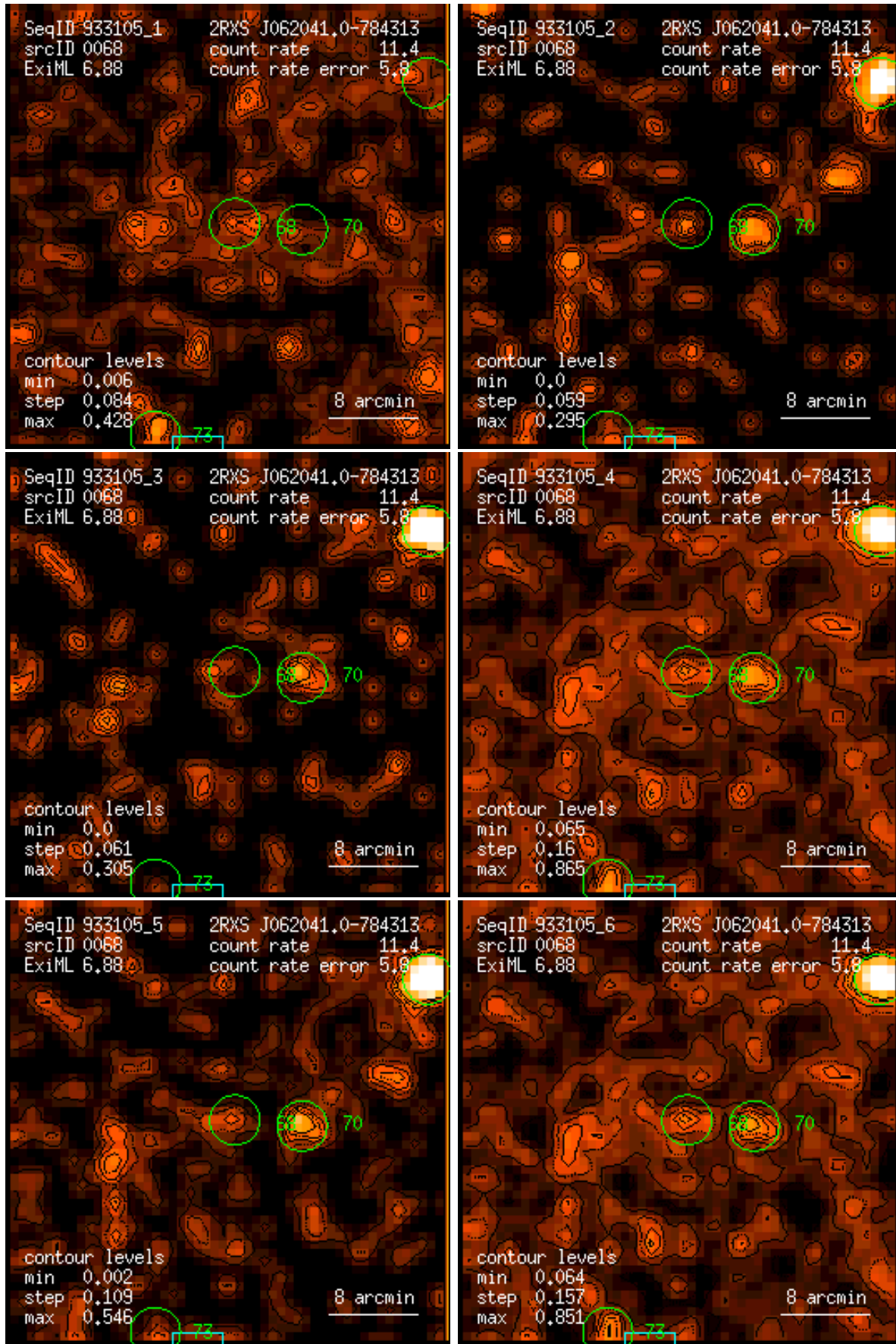
Figure 68: RASS 933105: detection 0068: band rate images, Gaussian filter: (1) PSPC channels 11 – 41, (2) 52 – 90, (3) 91 – 201, (4) 11 – 235, (5) 52 – 201, (6) 11 – 201. Broad band rates in counts/ks. Band rate contour levels in counts/ks/arcmin 2 .
