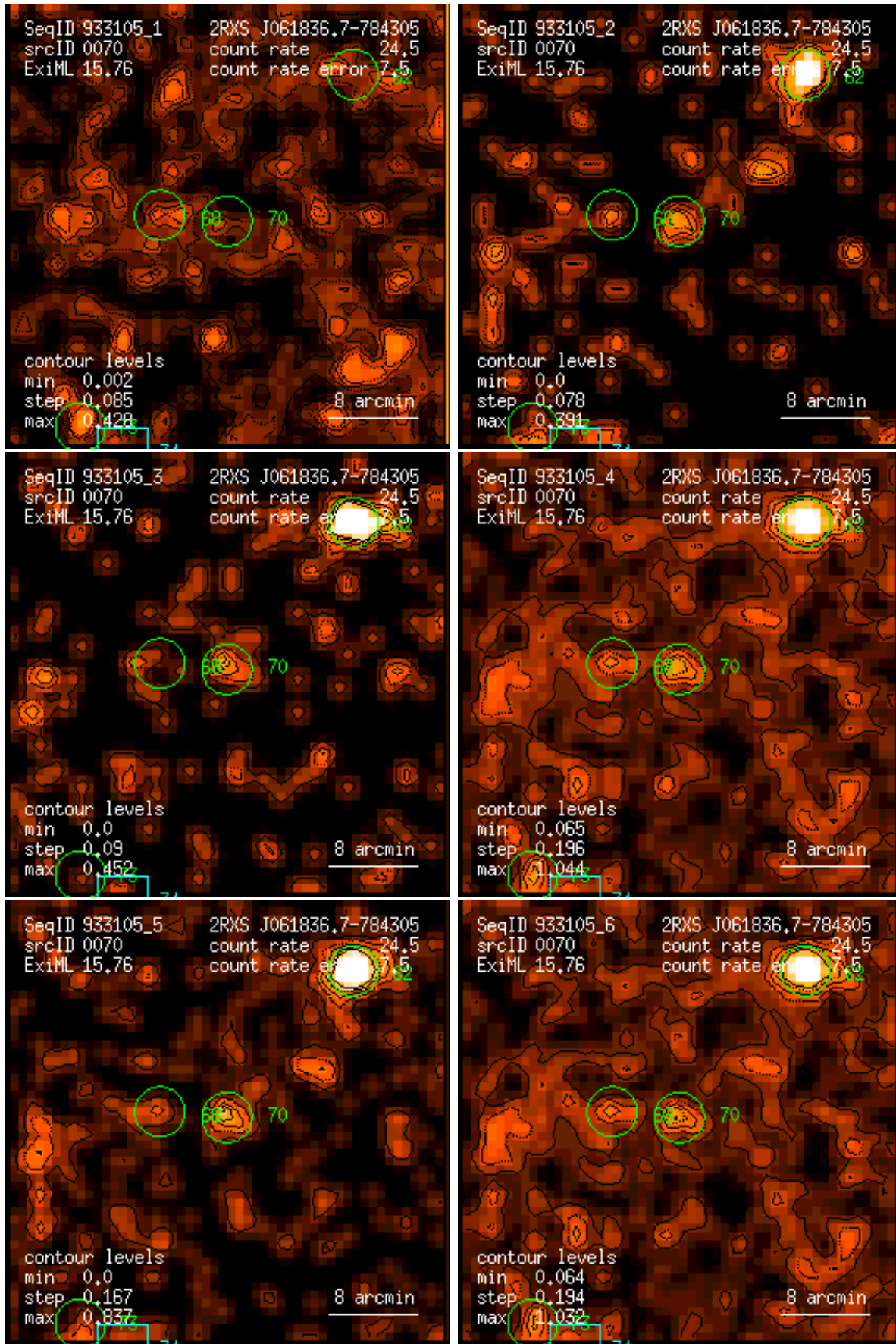
Figure 70: RASS 933105: detection 0070: band rate images, Gaussian filter: (1) PSPC channels 11 – 41, (2) 52 – 90, (3) 91 – 201, (4) 11 – 235, (5) 52 – 201, (6) 11 – 201. Broad band rates in counts/ks. Band rate contour levels in counts/ks/arcmin 2 .
