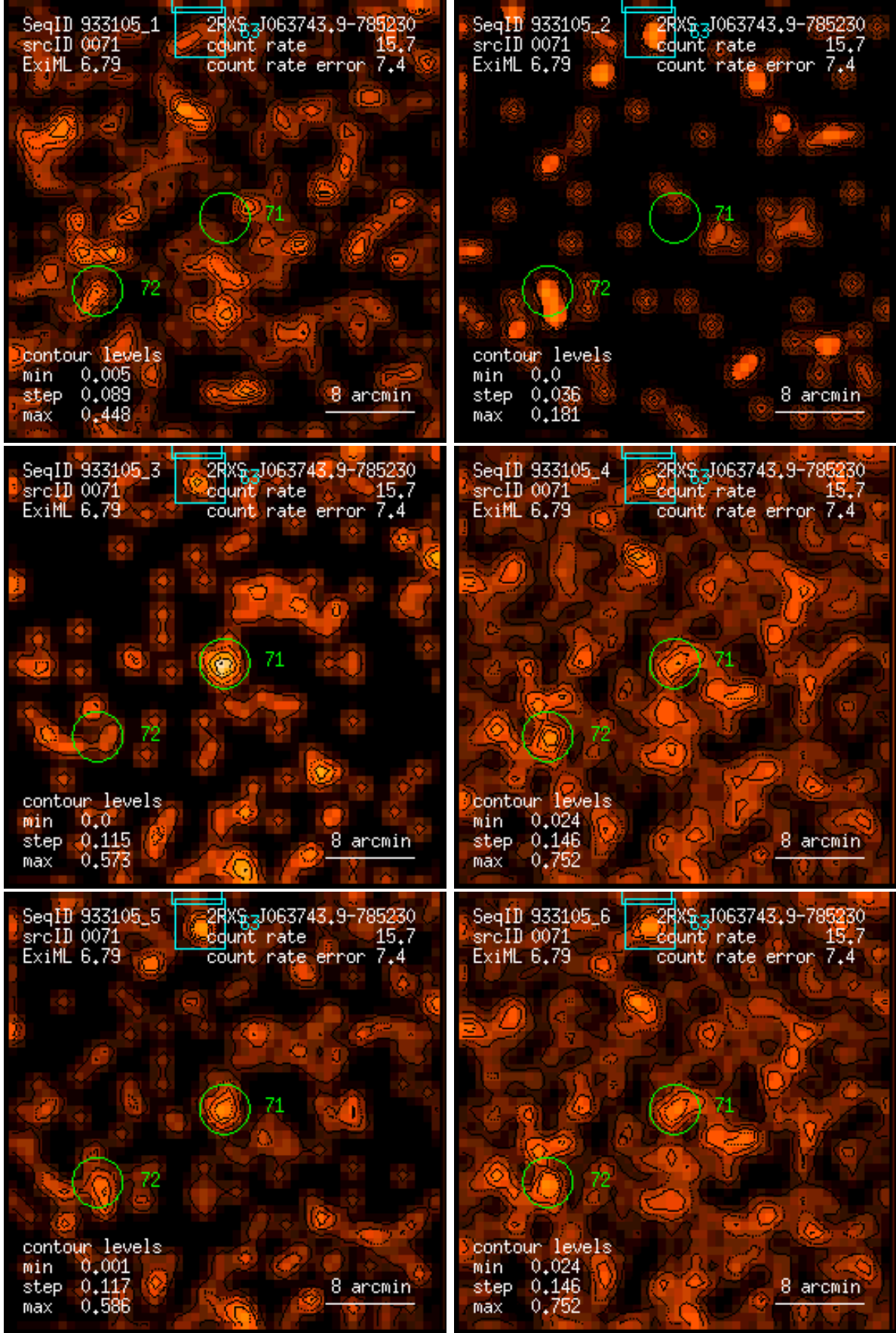
Figure 71: RASS 933105: detection 0071: band rate images, Gaussian filter: (1) PSPC channels 11 – 41, (2) 52 – 90, (3) 91 – 201, (4) 11 – 235, (5) 52 – 201, (6) 11 – 201. Broad band rates in counts/ks. Band rate contour levels in counts/ks/arcmin 2 .
