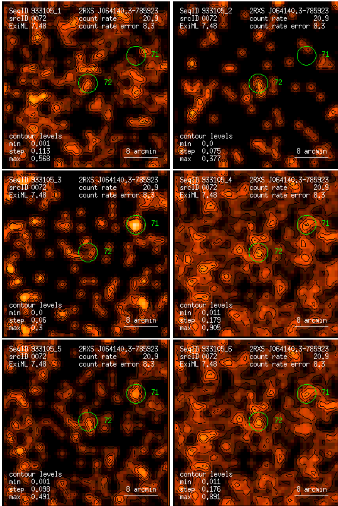
Figure 72: RASS 933105: detection 0072: band rate images, Gaussian filter: (1) PSPC channels 11 – 41, (2) 52 – 90, (3) 91 – 201, (4) 11 – 235, (5) 52 – 201, (6) 11 – 201. Broad band rates in counts/ks. Band rate contour levels in counts/ks/arcmin 2 .
