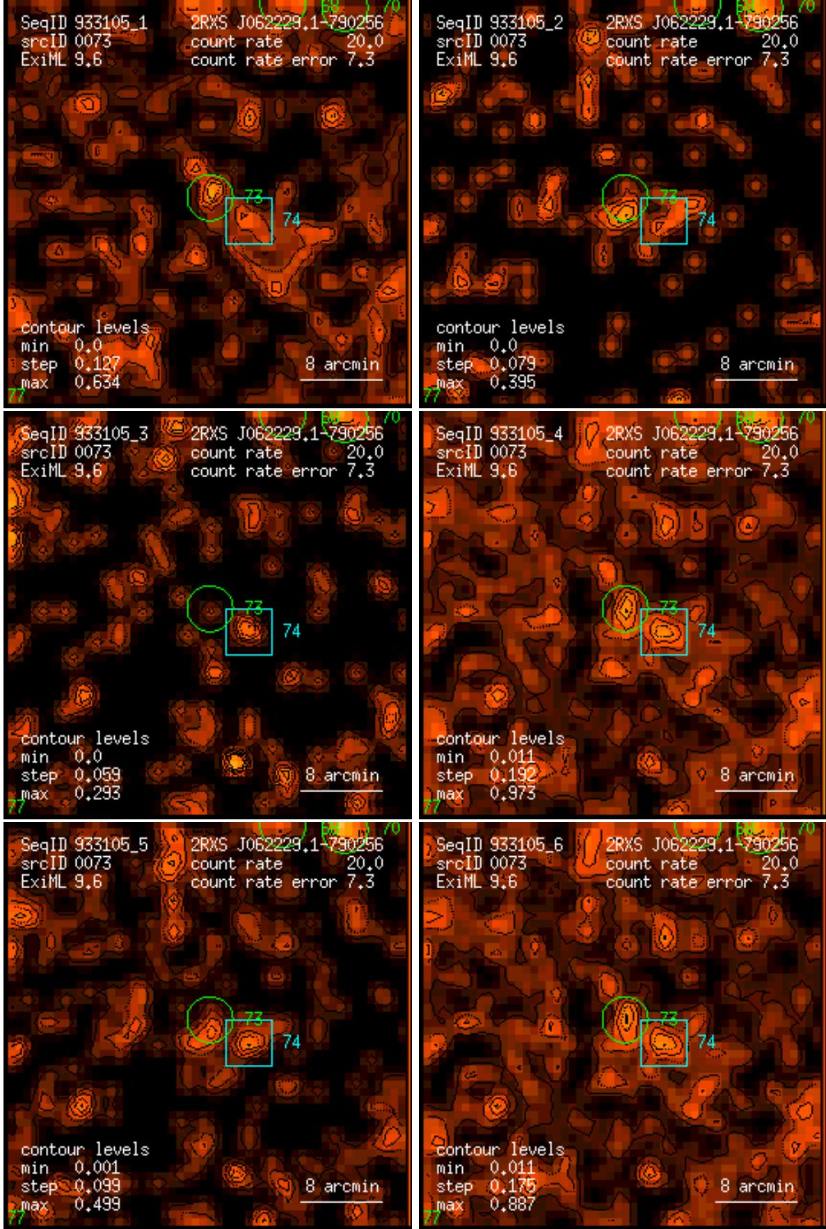
Figure 73: RASS 933105: detection 0073: band rate images, Gaussian filter: (1) PSPC channels 11 – 41, (2) 52 – 90, (3) 91 – 201, (4) 11 – 235, (5) 52 – 201, (6) 11 – 201. Broad band rates in counts/ks. Band rate contour levels in counts/ks/arcmin 2 .
