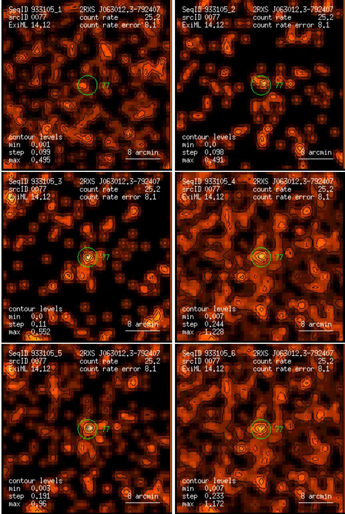
Figure 77: RASS 933105: detection 0077: band rate images, Gaussian filter: (1) PSPC channels 11 – 41, (2) 52 – 90, (3) 91 – 201, (4) 11 – 235, (5) 52 – 201, (6) 11 – 201. Broad band rates in counts/ks. Band rate contour levels in counts/ks/arcmin 2 .
