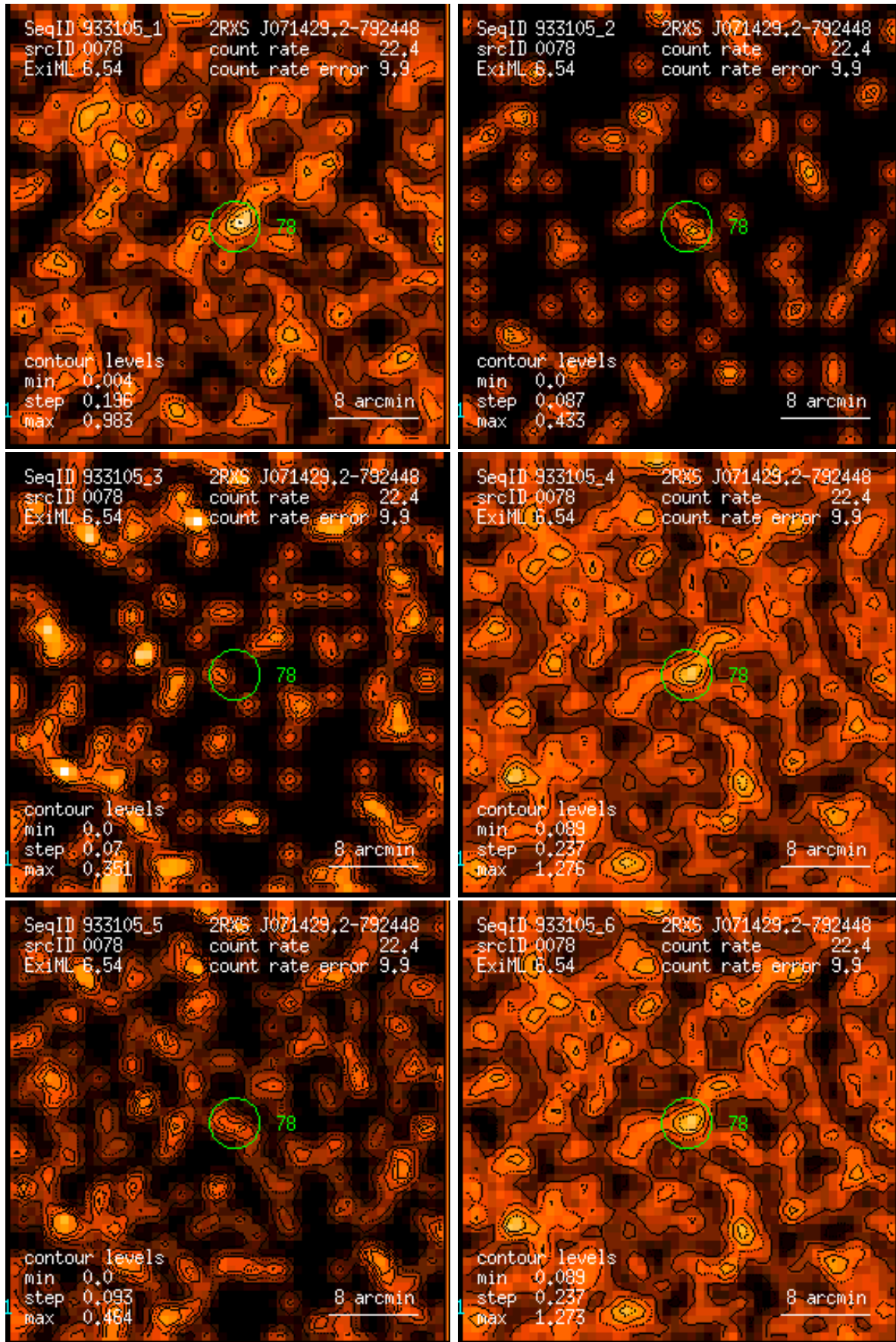
Figure 78: RASS 933105: detection 0078: band rate images, Gaussian filter: (1) PSPC channels 11 – 41, (2) 52 – 90, (3) 91 – 201, (4) 11 – 235, (5) 52 – 201, (6) 11 – 201. Broad band rates in counts/ks. Band rate contour levels in counts/ks/arcmin 2 .
