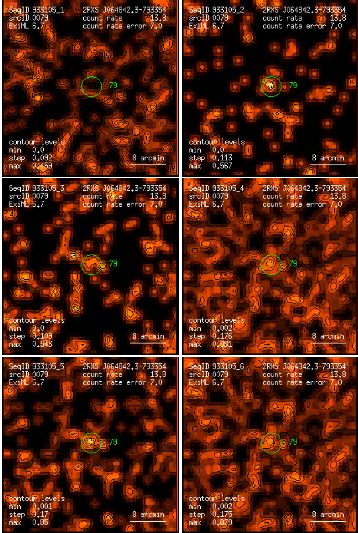
Figure 79: RASS 933105: detection 0079: band rate images, Gaussian filter: (1) PSPC channels 11 – 41, (2) 52 – 90, (3) 91 – 201, (4) 11 – 235, (5) 52 – 201, (6) 11 – 201. Broad band rates in counts/ks. Band rate contour levels in counts/ks/arcmin 2 .
