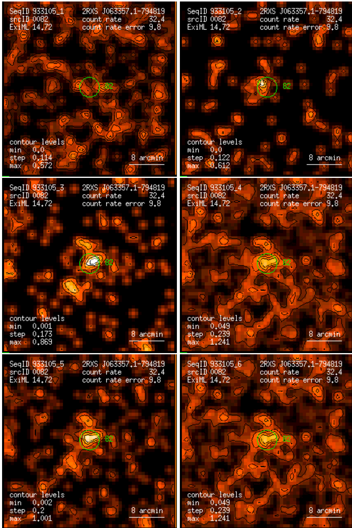
Figure 82: RASS 933105: detection 0082: band rate images, Gaussian filter: (1) PSPC channels 11 – 41, (2) 52 – 90, (3) 91 – 201, (4) 11 – 235, (5) 52 – 201, (6) 11 – 201. Broad band rates in counts/ks. Band rate contour levels in counts/ks/arcmin 2 .
