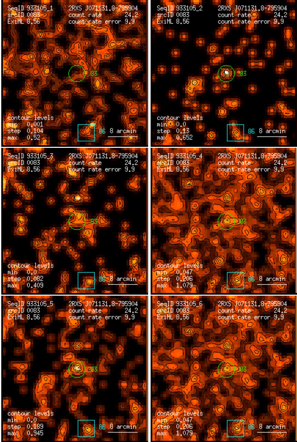
Figure 83: RASS 933105: detection 0083: band rate images, Gaussian filter: (1) PSPC channels 11 – 41, (2) 52 – 90, (3) 91 – 201, (4) 11 – 235, (5) 52 – 201, (6) 11 – 201. Broad band rates in counts/ks. Band rate contour levels in counts/ks/arcmin 2 .
