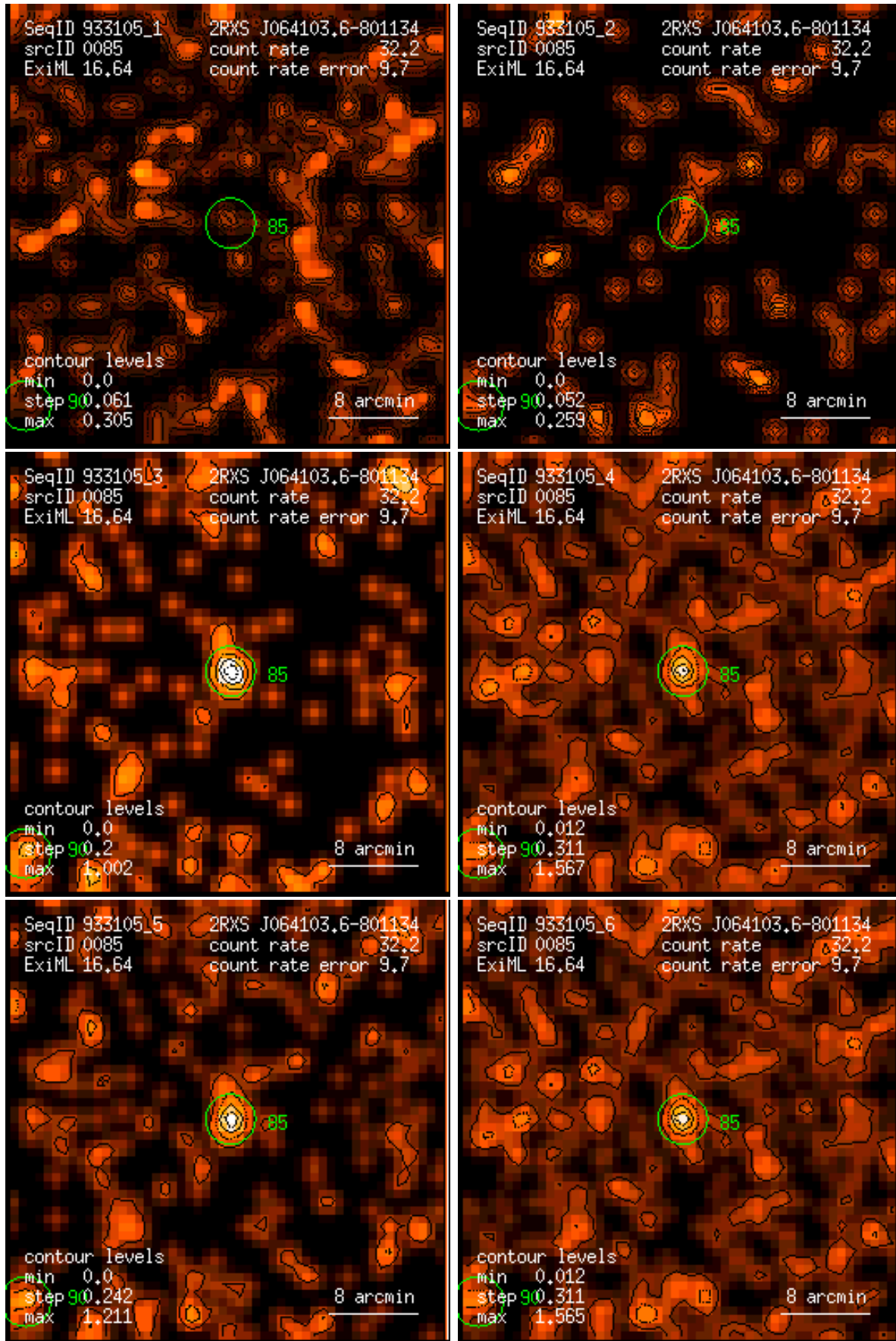
Figure 85: RASS 933105: detection 0085: band rate images, Gaussian filter: (1) PSPC channels 11 – 41, (2) 52 – 90, (3) 91 – 201, (4) 11 – 235, (5) 52 – 201, (6) 11 – 201. Broad band rates in counts/ks. Band rate contour levels in counts/ks/arcmin 2 .
