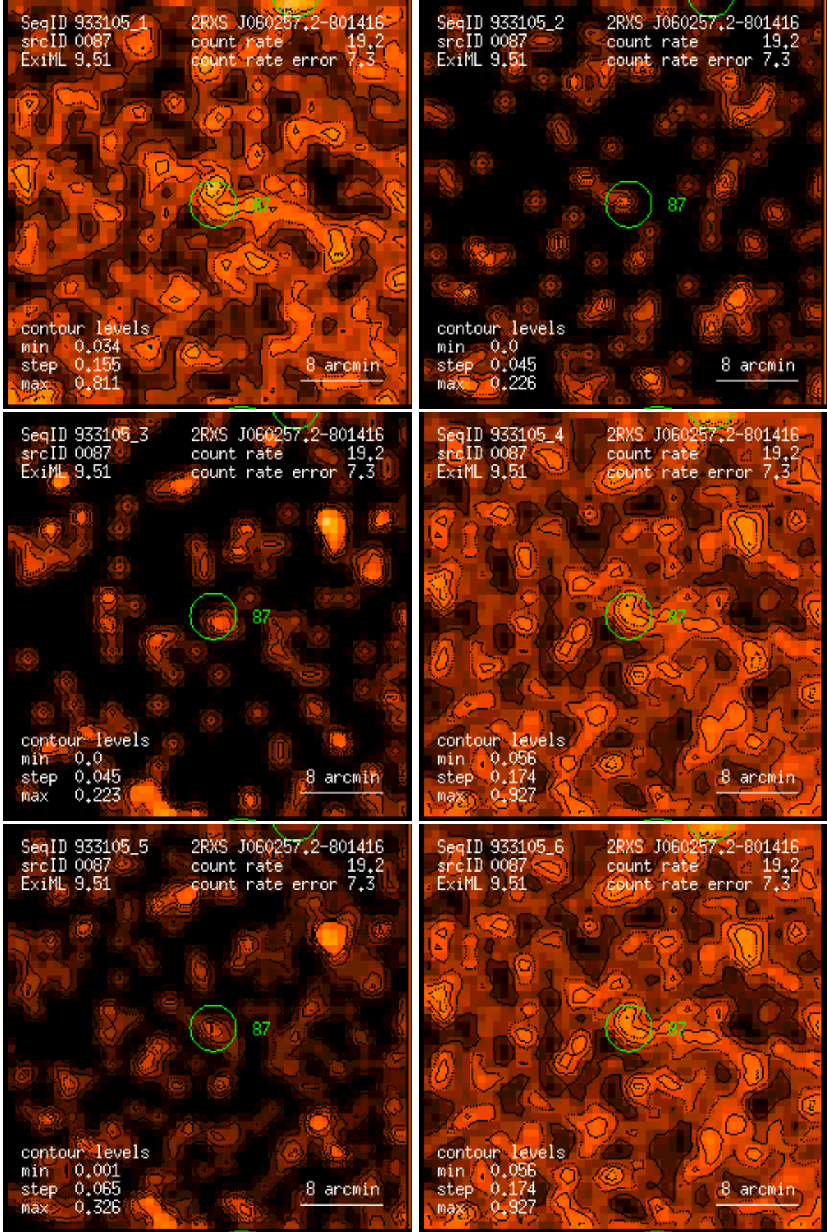
Figure 87: RASS 933105: detection 0087: band rate images, Gaussian filter: (1) PSPC channels 11 – 41, (2) 52 – 90, (3) 91 – 201, (4) 11 – 235, (5) 52 – 201, (6) 11 – 201. Broad band rates in counts/ks. Band rate contour levels in counts/ks/arcmin 2 .
