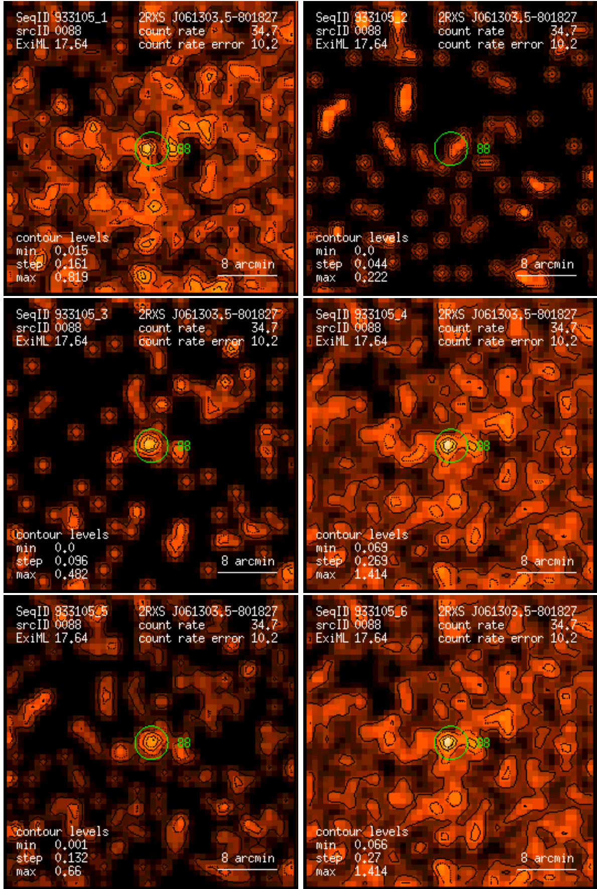
Figure 88: RASS 933105: detection 0088: band rate images, Gaussian filter: (1) PSPC channels 11 – 41, (2) 52 – 90, (3) 91 – 201, (4) 11 – 235, (5) 52 – 201, (6) 11 – 201. Broad band rates in counts/ks. Band rate contour levels in counts/ks/arcmin 2 .
