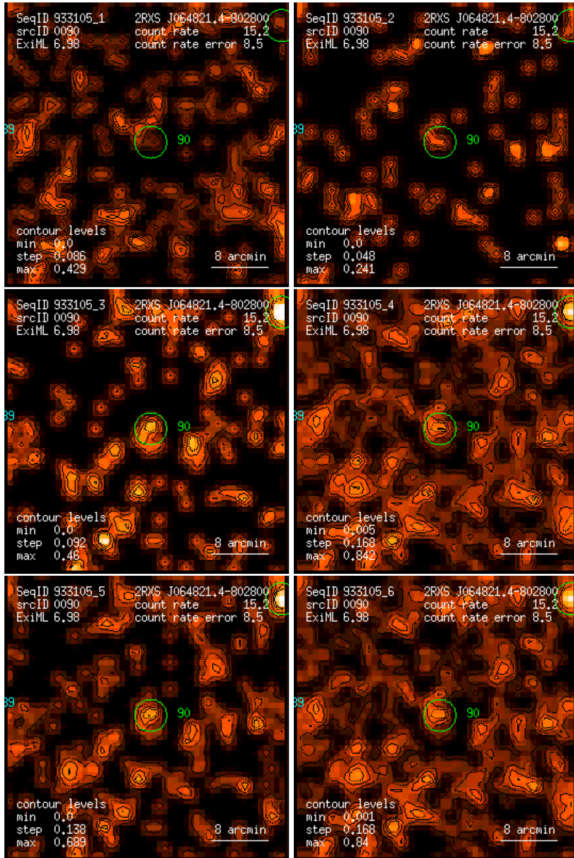
Figure 90: RASS 933105: detection 0090: band rate images, Gaussian filter: (1) PSPC channels 11 – 41, (2) 52 – 90, (3) 91 – 201, (4) 11 – 235, (5) 52 – 201, (6) 11 – 201. Broad band rates in counts/ks. Band rate contour levels in counts/ks/arcmin 2 .
