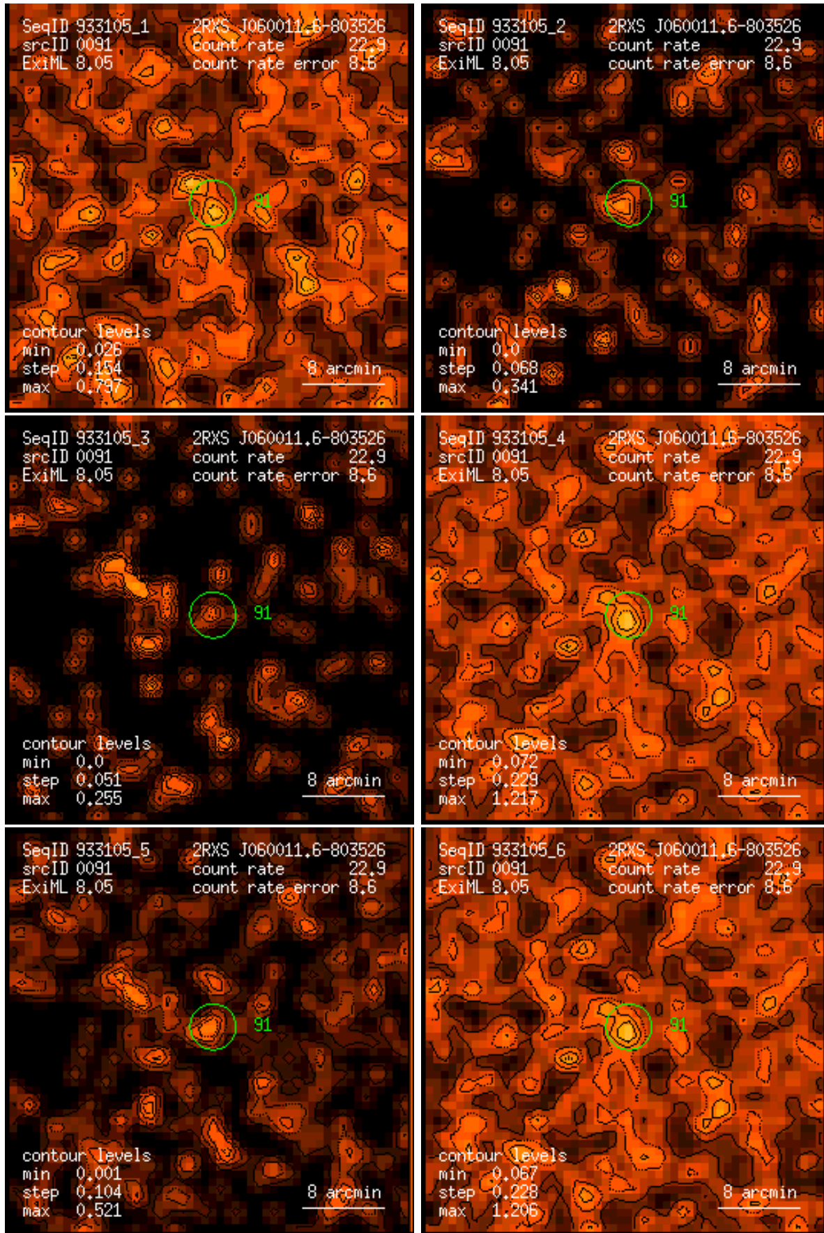
Figure 91: RASS 933105: detection 0091: band rate images, Gaussian filter: (1) PSPC channels 11 – 41, (2) 52 – 90, (3) 91 – 201, (4) 11 – 235, (5) 52 – 201, (6) 11 – 201. Broad band rates in counts/ks. Band rate contour levels in counts/ks/arcmin 2 .
