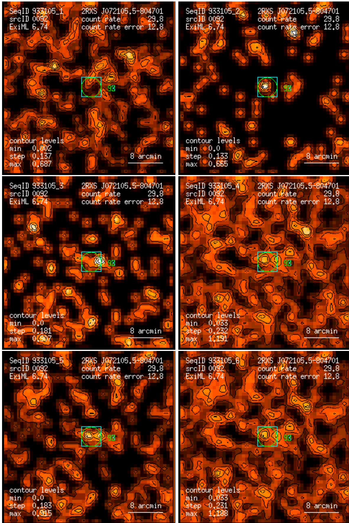
Figure 92: RASS 933105: detection 0092: band rate images, Gaussian filter: (1) PSPC channels 11 – 41, (2) 52 – 90, (3) 91 – 201, (4) 11 – 235, (5) 52 – 201, (6) 11 – 201. Broad band rates in counts/ks. Band rate contour levels in counts/ks/arcmin 2 .
