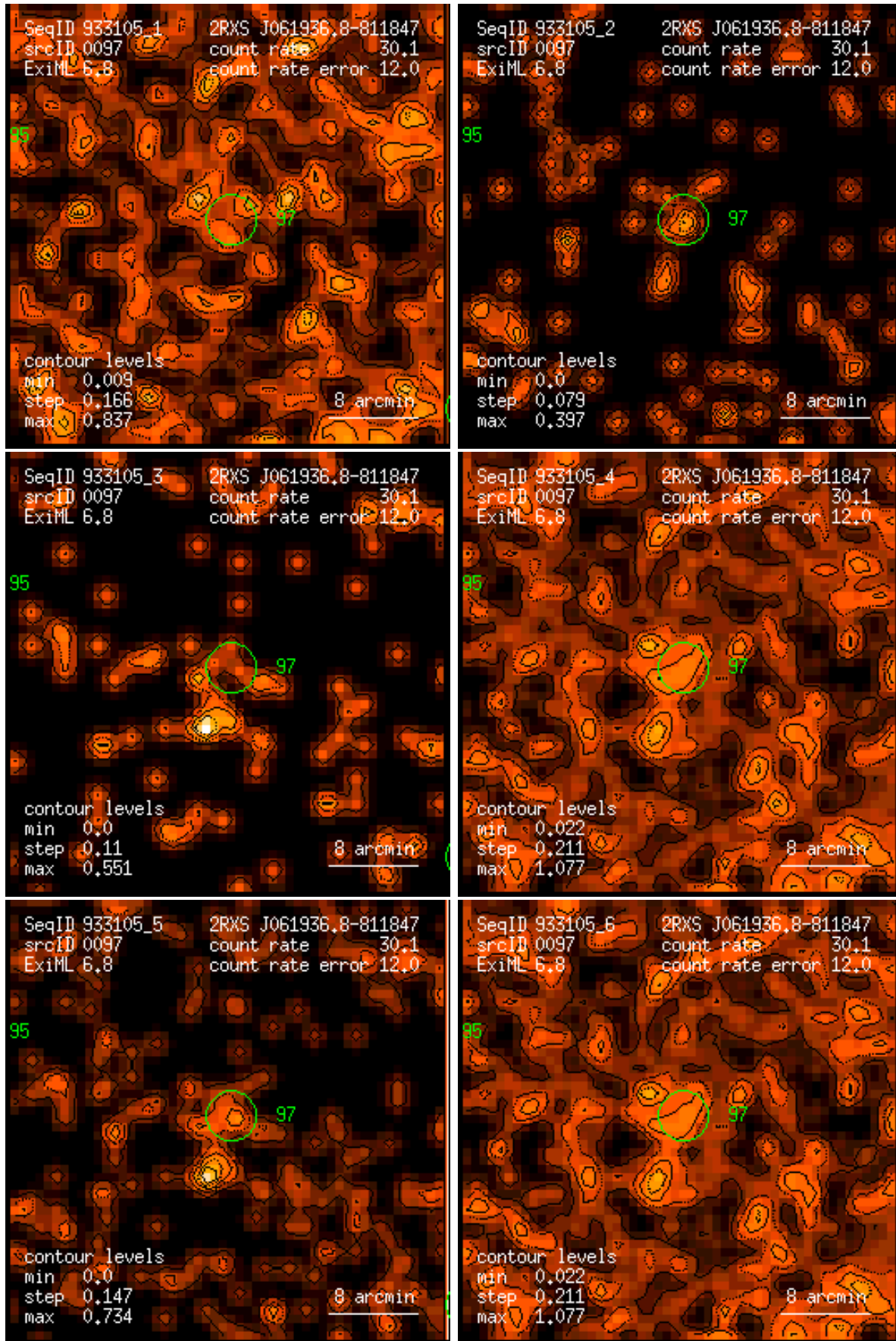
Figure 97: RASS 933105: detection 0097: band rate images, Gaussian filter: (1) PSPC channels 11 – 41, (2) 52 – 90, (3) 91 – 201, (4) 11 – 235, (5) 52 – 201, (6) 11 – 201. Broad band rates in counts/ks. Band rate contour levels in counts/ks/arcmin 2 .
