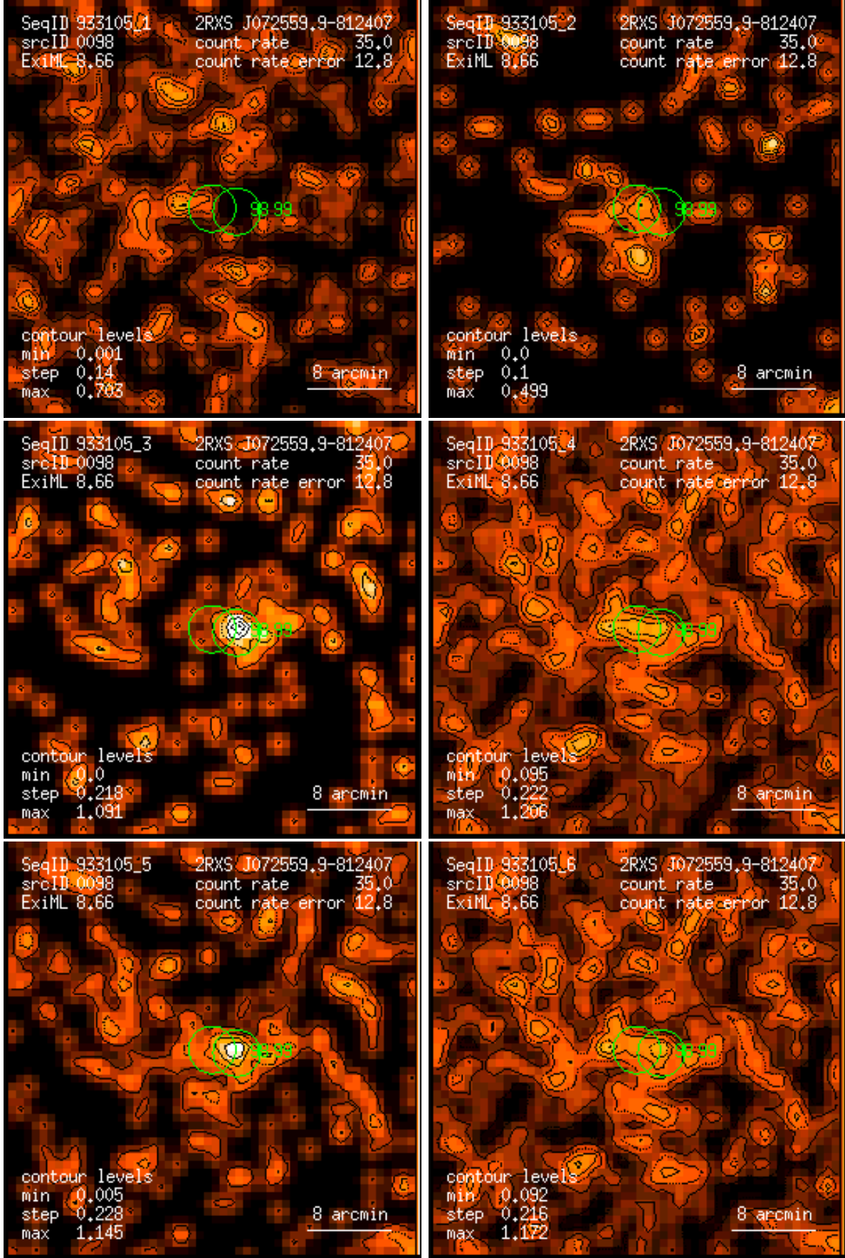
Figure 98: RASS 933105: detection 0098: band rate images, Gaussian filter: (1) PSPC channels 11 – 41, (2) 52 – 90, (3) 91 – 201, (4) 11 – 235, (5) 52 – 201, (6) 11 – 201. Broad band rates in counts/ks. Band rate contour levels in counts/ks/arcmin 2 .
