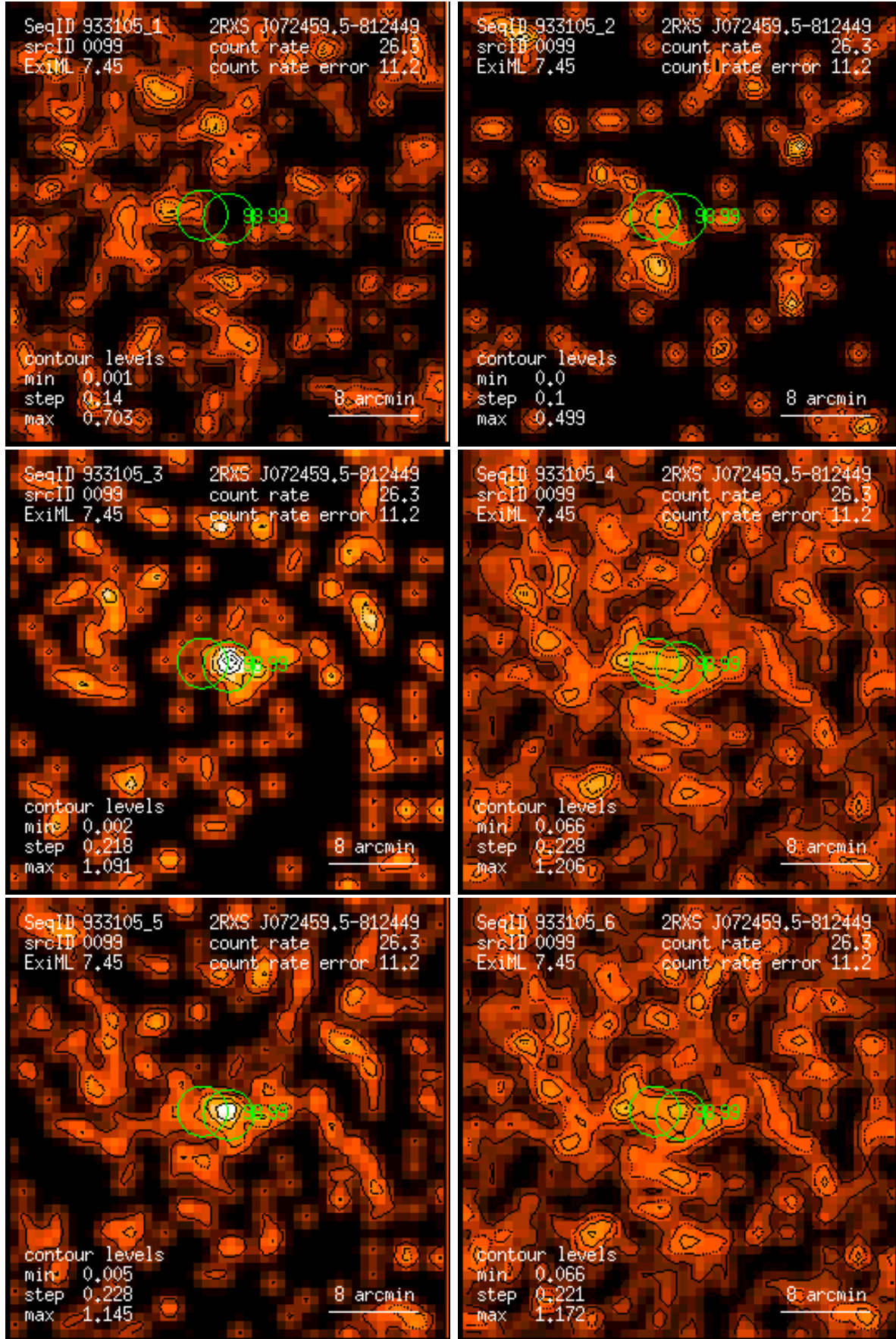
Figure 99: RASS 933105: detection 0099: band rate images, Gaussian filter: (1) PSPC channels 11 – 41, (2) 52 – 90, (3) 91 – 201, (4) 11 – 235, (5) 52 – 201, (6) 11 – 201. Broad band rates in counts/ks. Band rate contour levels in counts/ks/arcmin 2 .
