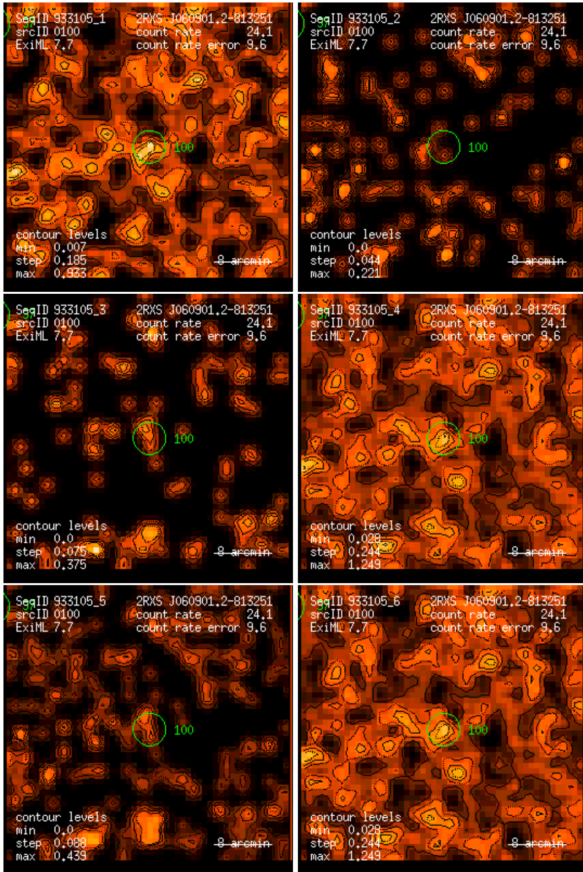
Figure 100: RASS 933105: detection 0100: band rate images, Gaussian filter: (1) PSPC channels 11 – 41, (2) 52 – 90, (3) 91 – 201, (4) 11 – 235, (5) 52 – 201, (6) 11 – 201. Broad band rates in counts/ks. Band rate contour levels in counts/ks/arcmin 2 .
