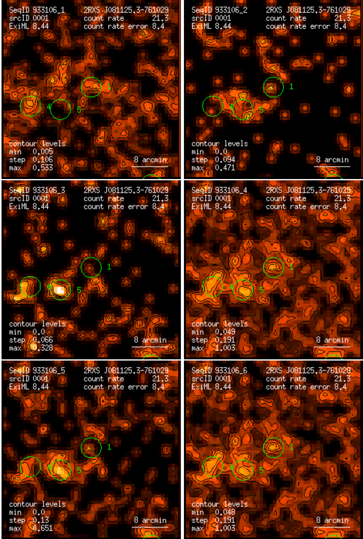
Figure 1: RASS 933106: detection 0001: band rate images, Gaussian filter: (1) PSPC channels 11 – 41, (2) 52 – 90, (3) 91 – 201, (4) 11 – 235, (5) 52 – 201, (6) 11 – 201. Broad band rates in counts/ks. Band rate contour levels in counts/ks/arcmin 2 .
