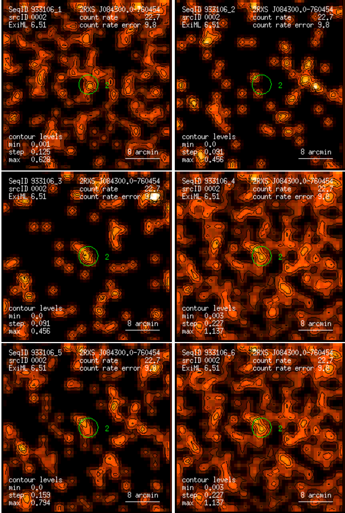
Figure 2: RASS 933106: detection 0002: band rate images, Gaussian filter: (1) PSPC channels 11 – 41, (2) 52 – 90, (3) 91 – 201, (4) 11 – 235, (5) 52 – 201, (6) 11 – 201. Broad band rates in counts/ks. Band rate contour levels in counts/ks/arcmin 2 .
