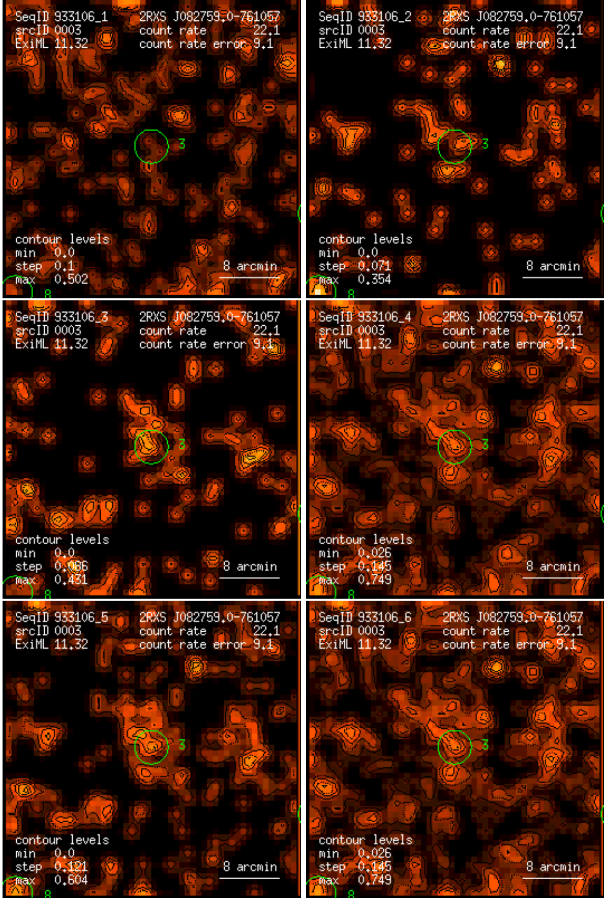
Figure 3: RASS 933106: detection 0003: band rate images, Gaussian filter: (1) PSPC channels 11 – 41, (2) 52 – 90, (3) 91 – 201, (4) 11 – 235, (5) 52 – 201, (6) 11 – 201. Broad band rates in counts/ks. Band rate contour levels in counts/ks/arcmin 2 .
