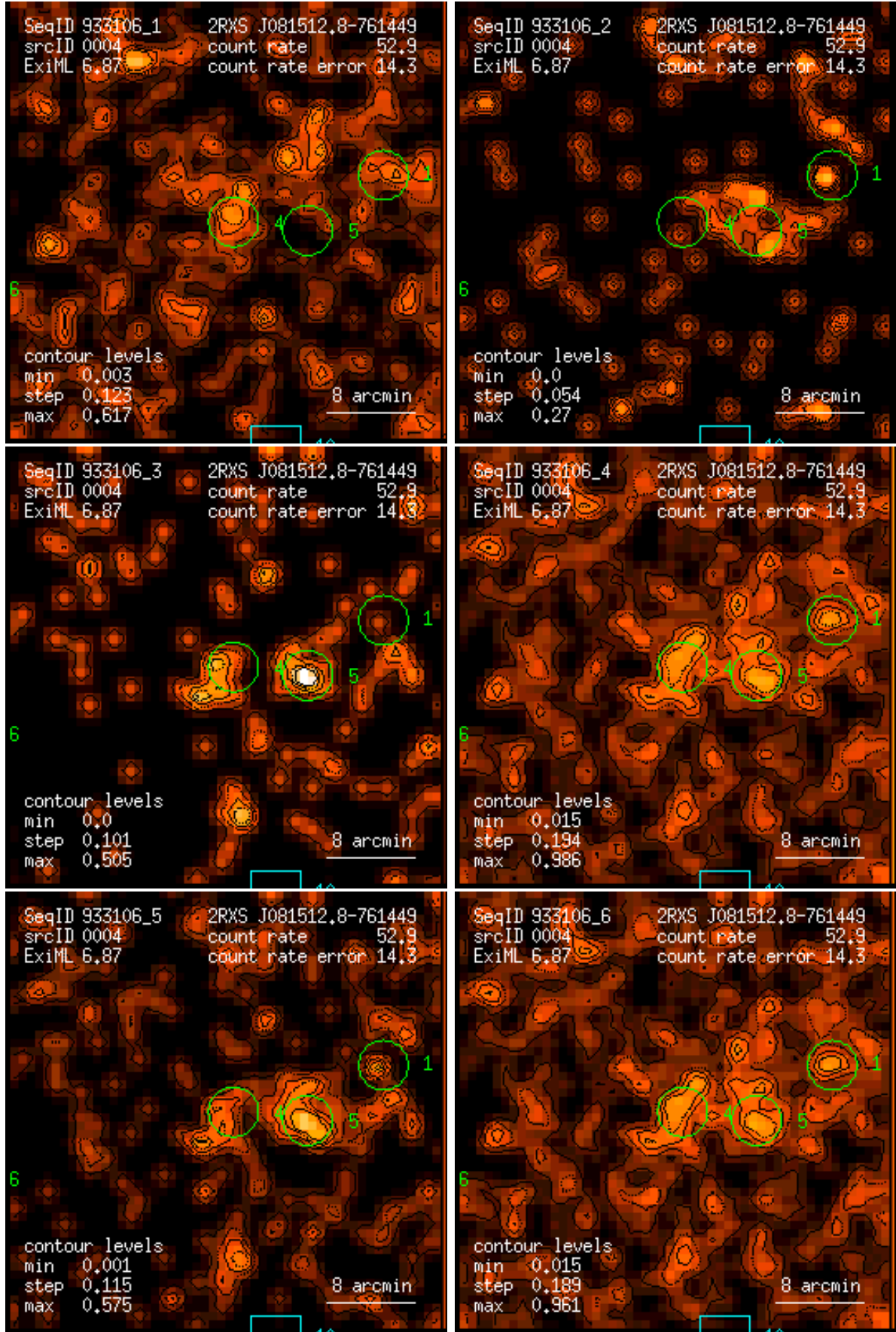
Figure 4: RASS 933106: detection 0004: band rate images, Gaussian filter: (1) PSPC channels 11 – 41, (2) 52 – 90, (3) 91 – 201, (4) 11 – 235, (5) 52 – 201, (6) 11 – 201. Broad band rates in counts/ks. Band rate contour levels in counts/ks/arcmin 2 .
