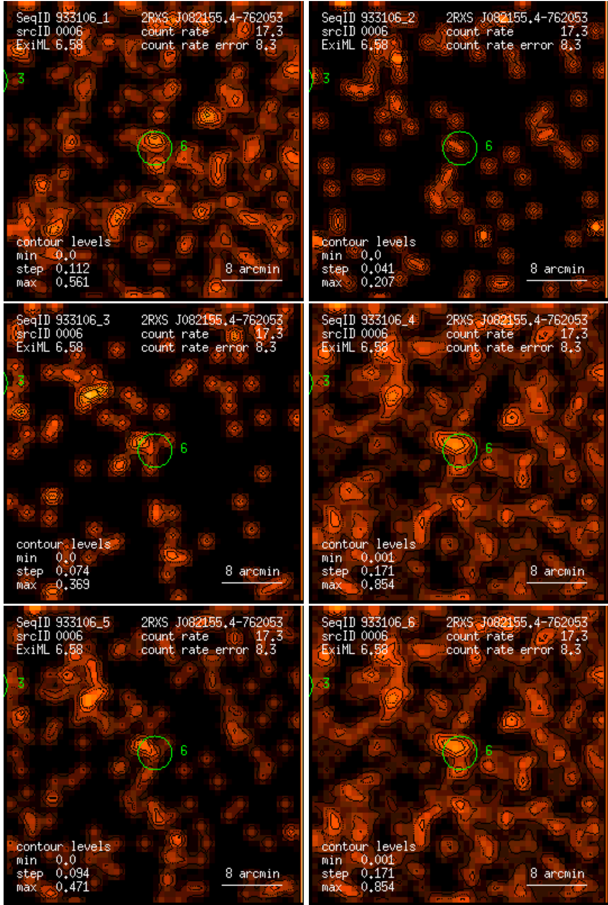
Figure 6: RASS 933106: detection 0006: band rate images, Gaussian filter: (1) PSPC channels 11 – 41, (2) 52 – 90, (3) 91 – 201, (4) 11 – 235, (5) 52 – 201, (6) 11 – 201. Broad band rates in counts/ks. Band rate contour levels in counts/ks/arcmin 2 .
