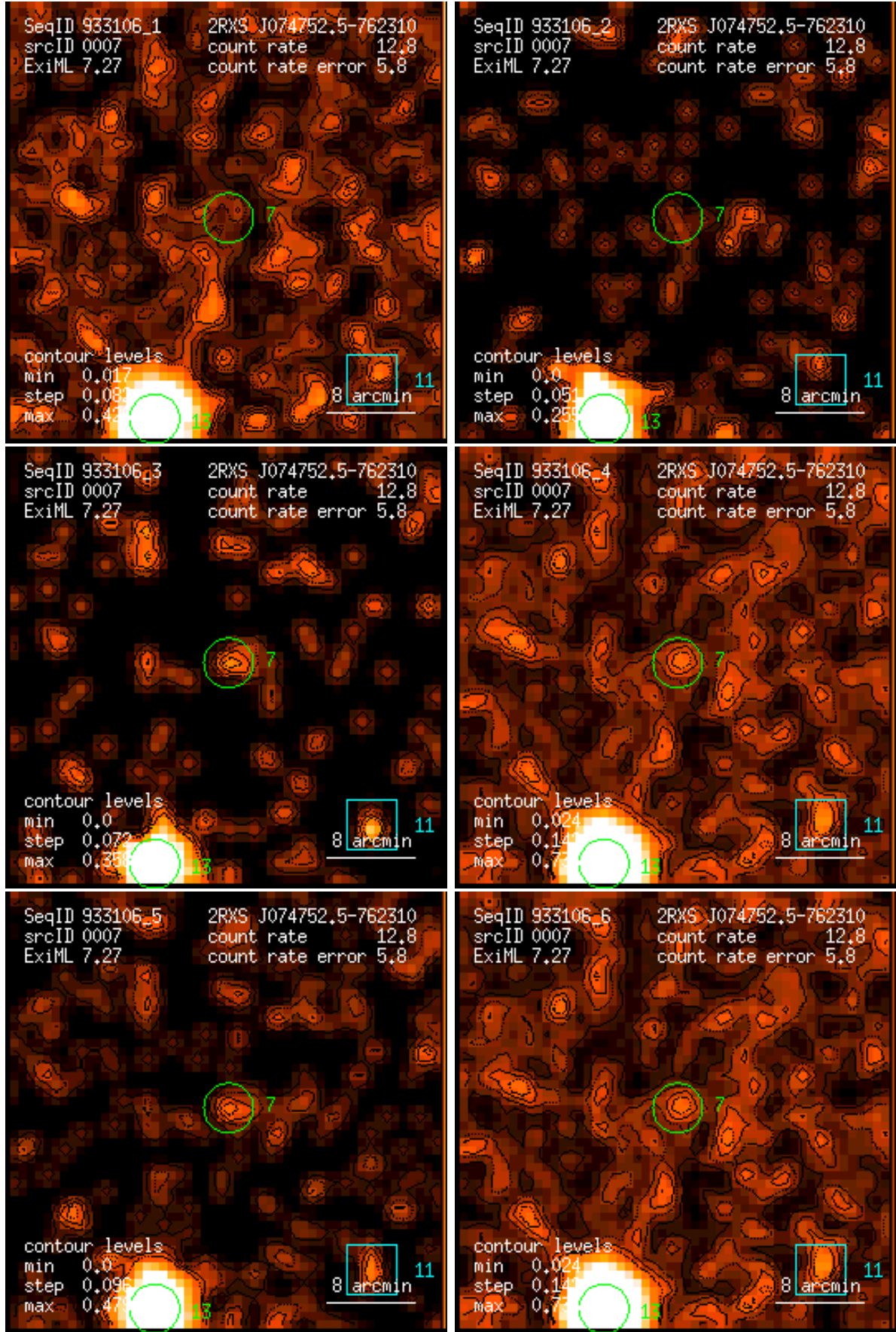
Figure 7: RASS 933106: detection 0007: band rate images, Gaussian filter: (1) PSPC channels 11 – 41, (2) 52 – 90, (3) 91 – 201, (4) 11 – 235, (5) 52 – 201, (6) 11 – 201. Broad band rates in counts/ks. Band rate contour levels in counts/ks/arcmin 2 .
