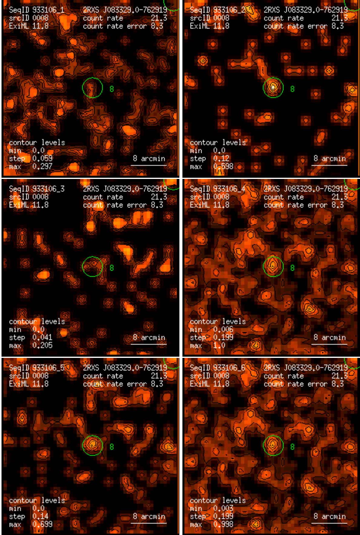
Figure 8: RASS 933106: detection 0008: band rate images, Gaussian filter: (1) PSPC channels 11 – 41, (2) 52 – 90, (3) 91 – 201, (4) 11 – 235, (5) 52 – 201, (6) 11 – 201. Broad band rates in counts/ks. Band rate contour levels in counts/ks/arcmin 2 .
