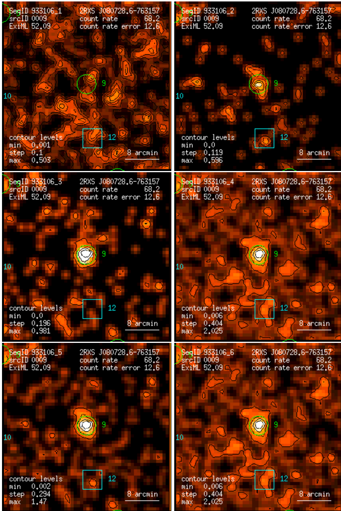
Figure 9: RASS 933106: detection 0009: band rate images, Gaussian filter: (1) PSPC channels 11 – 41, (2) 52 – 90, (3) 91 – 201, (4) 11 – 235, (5) 52 – 201, (6) 11 – 201. Broad band rates in counts/ks. Band rate contour levels in counts/ks/arcmin 2 .
