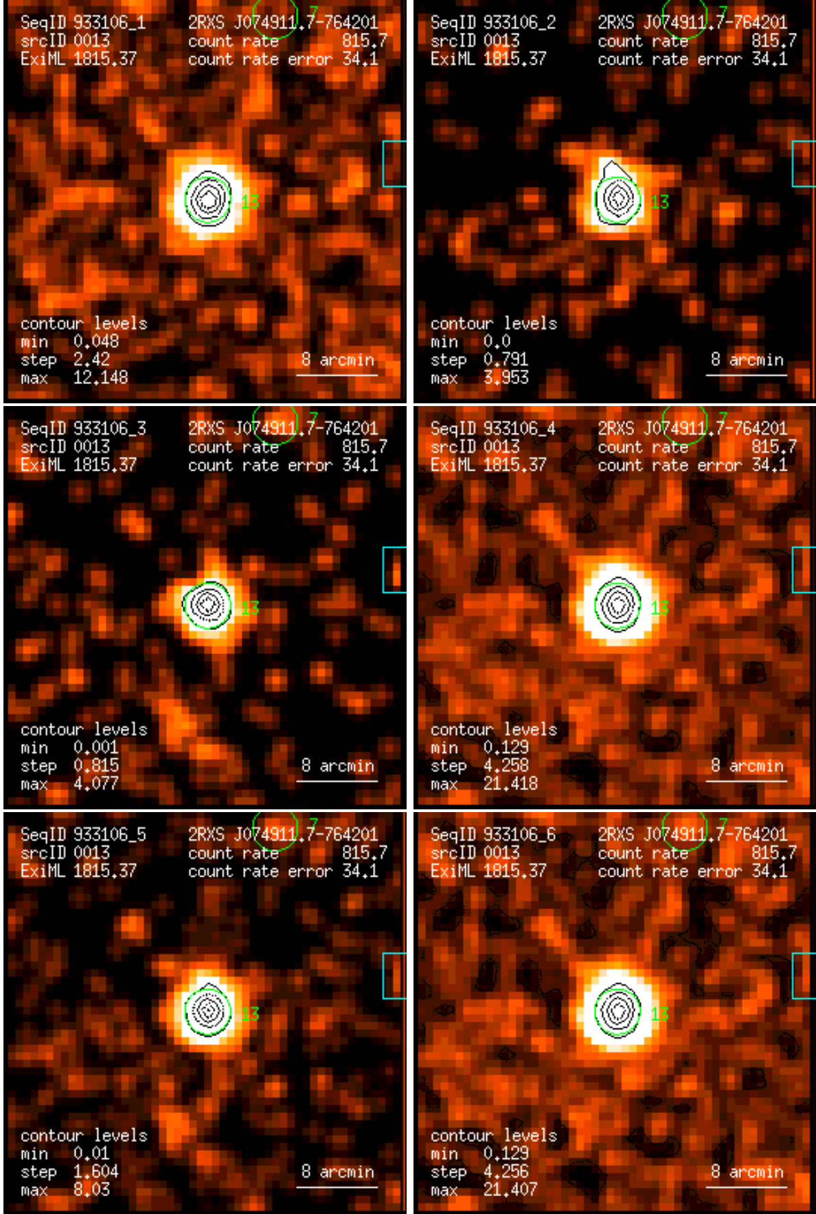
Figure 13: RASS 933106: detection 0013: band rate images, Gaussian filter: (1) PSPC channels 11 – 41, (2) 52 – 90, (3) 91 – 201, (4) 11 – 235, (5) 52 – 201, (6) 11 – 201. Broad band rates in counts/ks. Band rate contour levels in counts/ks/arcmin 2 .
