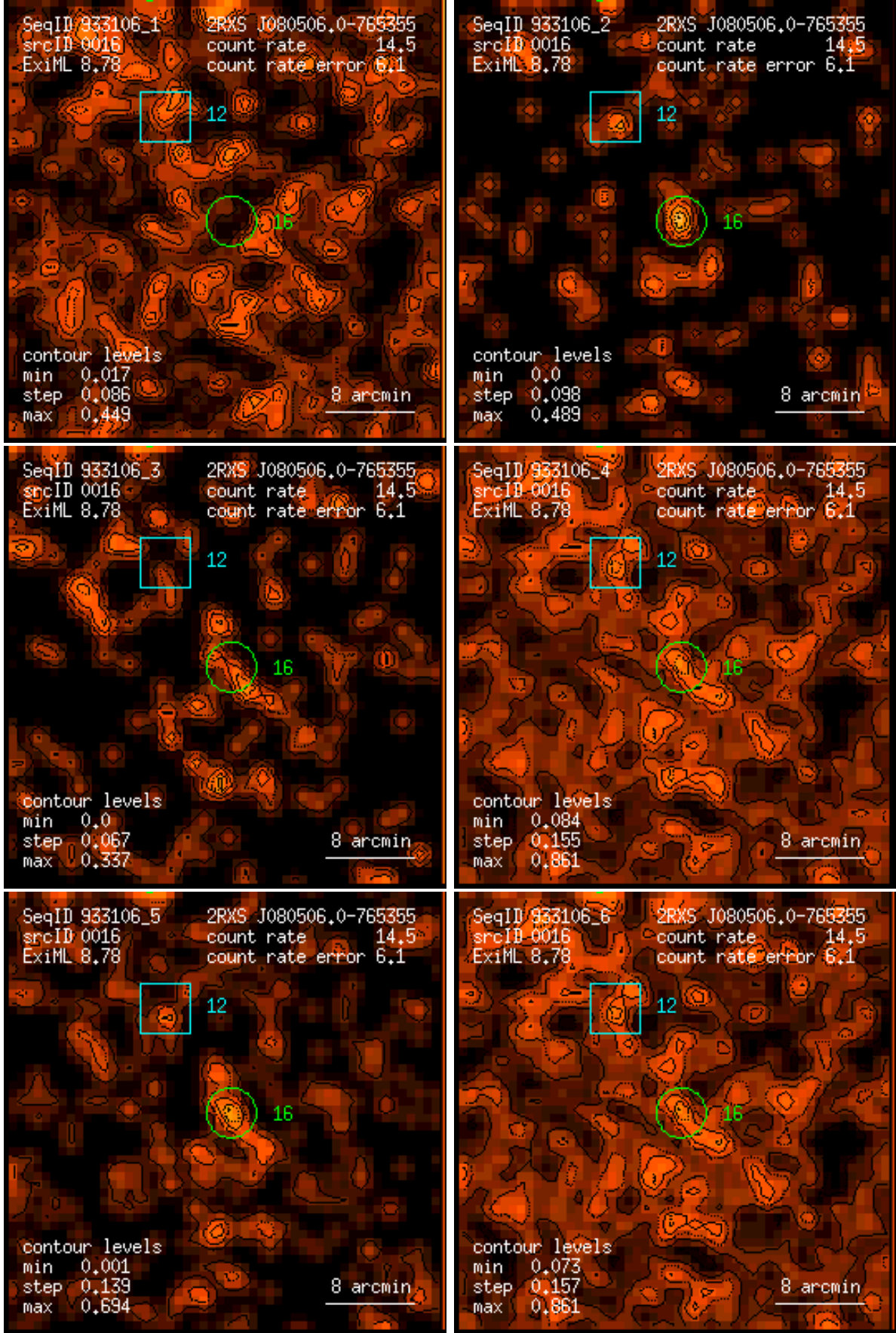
Figure 16: RASS 933106: detection 0016: band rate images, Gaussian filter: (1) PSPC channels 11 – 41, (2) 52 – 90, (3) 91 – 201, (4) 11 – 235, (5) 52 – 201, (6) 11 – 201. Broad band rates in counts/ks. Band rate contour levels in counts/ks/arcmin 2 .
