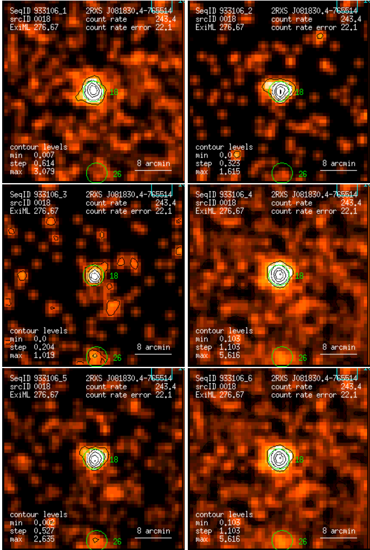
Figure 18: RASS 933106: detection 0018: band rate images, Gaussian filter: (1) PSPC channels 11 – 41, (2) 52 – 90, (3) 91 – 201, (4) 11 – 235, (5) 52 – 201, (6) 11 – 201. Broad band rates in counts/ks. Band rate contour levels in counts/ks/arcmin 2 .
