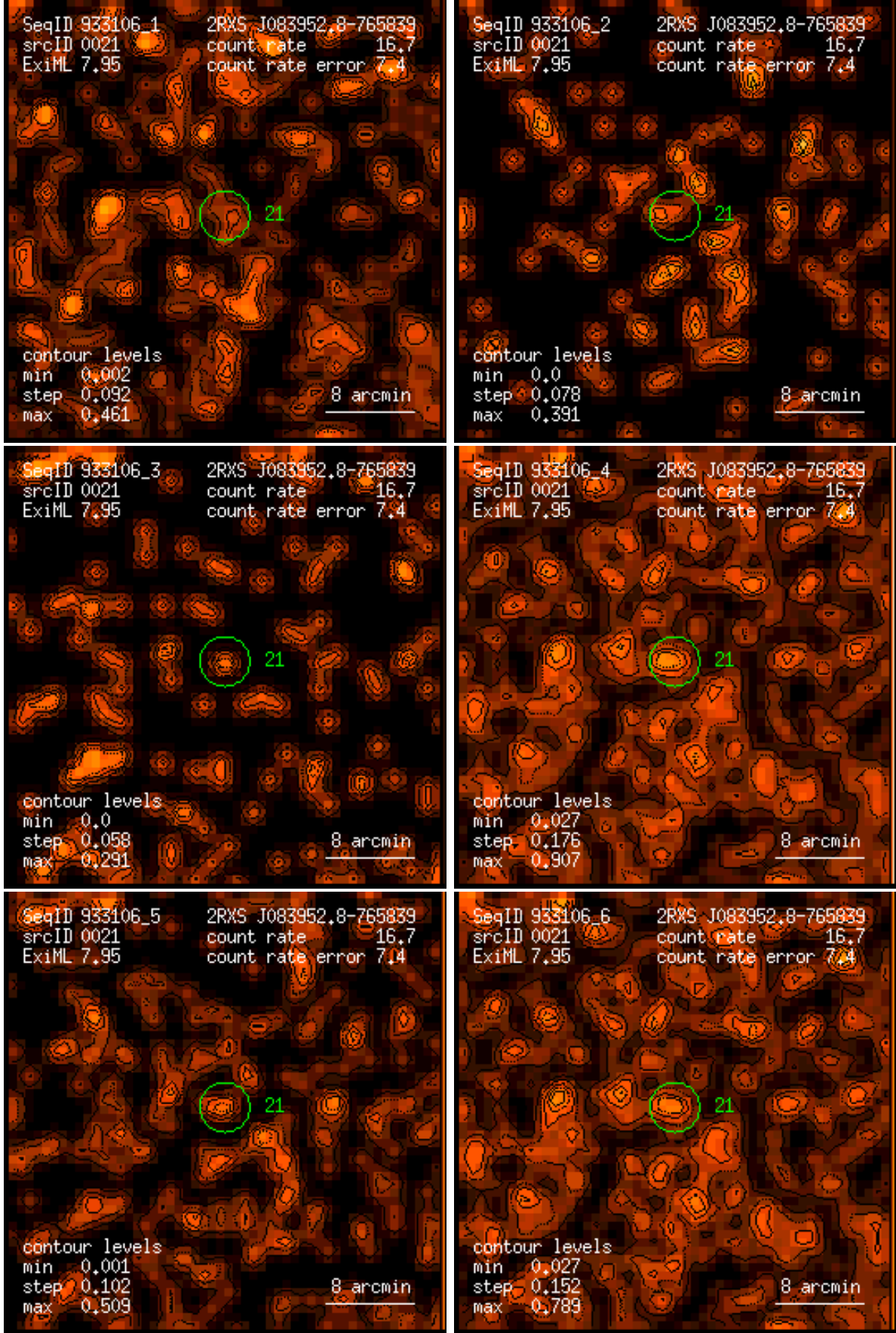
Figure 21: RASS 933106: detection 0021: band rate images, Gaussian filter: (1) PSPC channels 11 – 41, (2) 52 – 90, (3) 91 – 201, (4) 11 – 235, (5) 52 – 201, (6) 11 – 201. Broad band rates in counts/ks. Band rate contour levels in counts/ks/arcmin 2 .
