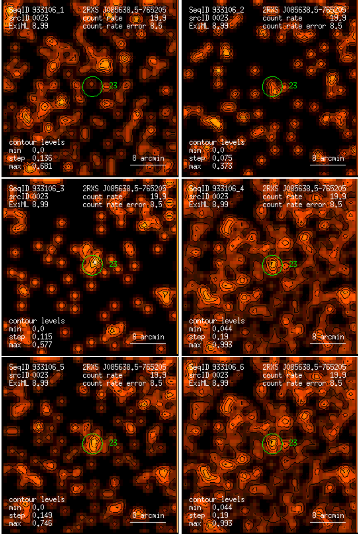
Figure 23: RASS 933106: detection 0023: band rate images, Gaussian filter: (1) PSPC channels 11 – 41, (2) 52 – 90, (3) 91 – 201, (4) 11 – 235, (5) 52 – 201, (6) 11 – 201. Broad band rates in counts/ks. Band rate contour levels in counts/ks/arcmin 2 .
