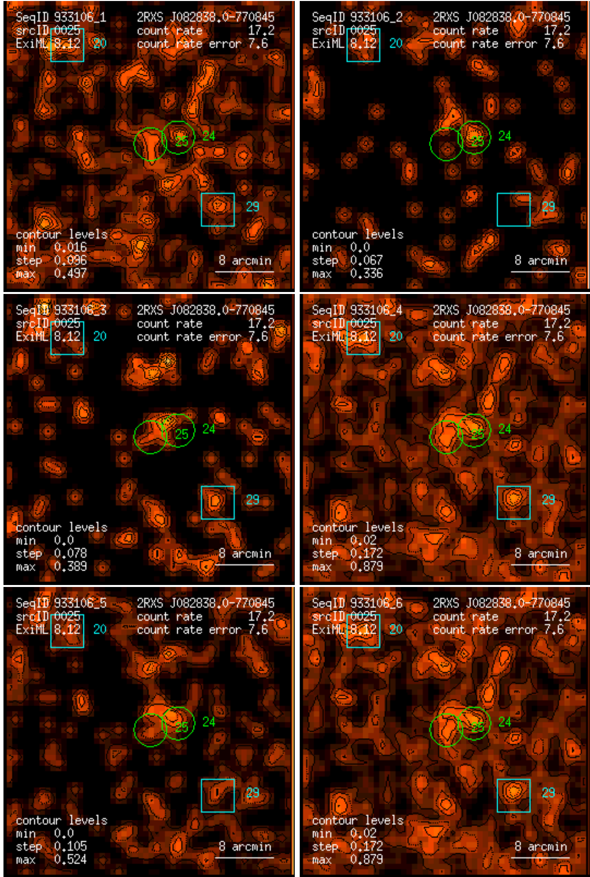
Figure 25: RASS 933106: detection 0025: band rate images, Gaussian filter: (1) PSPC channels 11 – 41, (2) 52 – 90, (3) 91 – 201, (4) 11 – 235, (5) 52 – 201, (6) 11 – 201. Broad band rates in counts/ks. Band rate contour levels in counts/ks/arcmin 2 .
