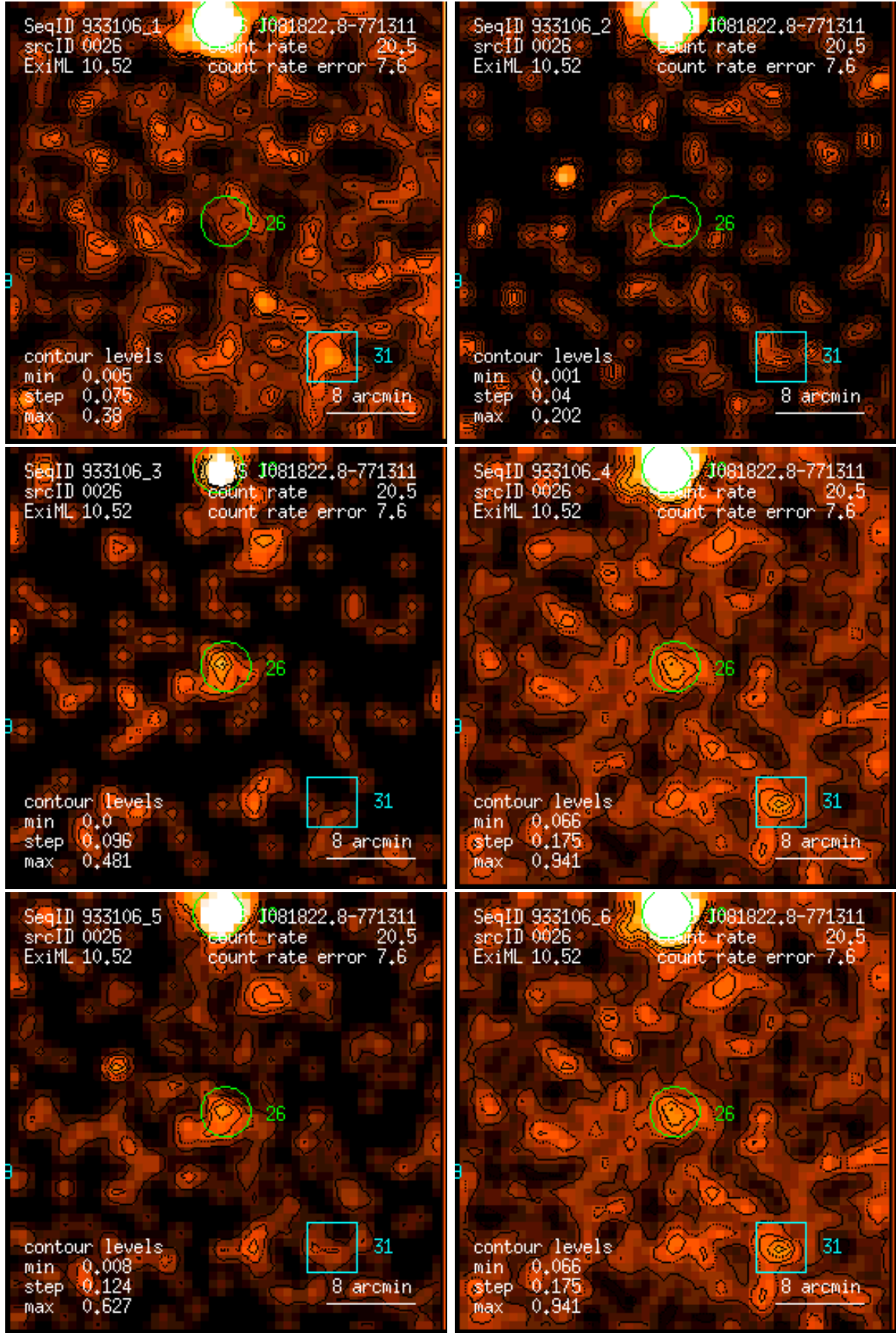
Figure 26: RASS 933106: detection 0026: band rate images, Gaussian filter: (1) PSPC channels 11 – 41, (2) 52 – 90, (3) 91 – 201, (4) 11 – 235, (5) 52 – 201, (6) 11 – 201. Broad band rates in counts/ks. Band rate contour levels in counts/ks/arcmin 2 .
