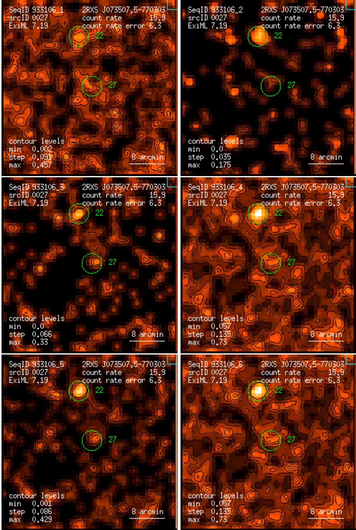
Figure 27: RASS 933106: detection 0027: band rate images, Gaussian filter: (1) PSPC channels 11 – 41, (2) 52 – 90, (3) 91 – 201, (4) 11 – 235, (5) 52 – 201, (6) 11 – 201. Broad band rates in counts/ks. Band rate contour levels in counts/ks/arcmin 2 .
