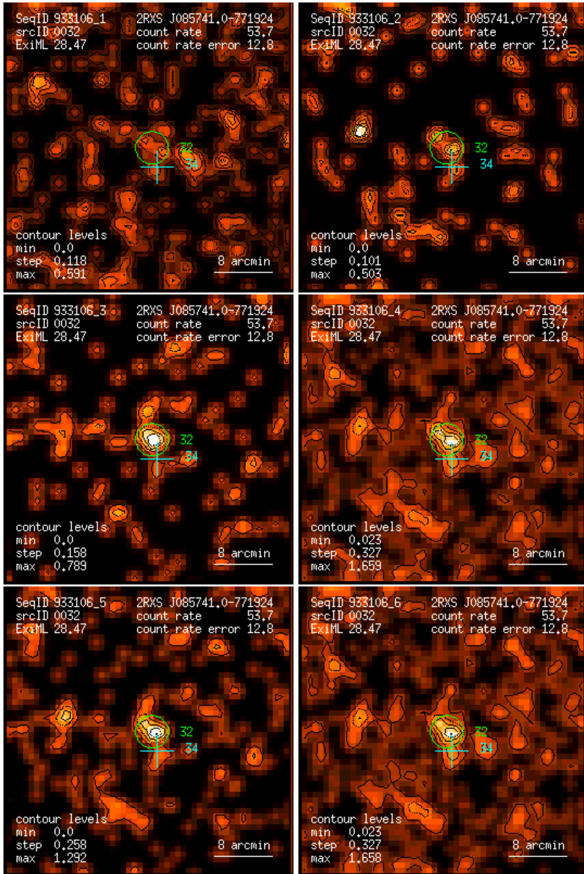
Figure 32: RASS 933106: detection 0032: band rate images, Gaussian filter: (1) PSPC channels 11 – 41, (2) 52 – 90, (3) 91 – 201, (4) 11 – 235, (5) 52 – 201, (6) 11 – 201. Broad band rates in counts/ks. Band rate contour levels in counts/ks/arcmin 2 .
