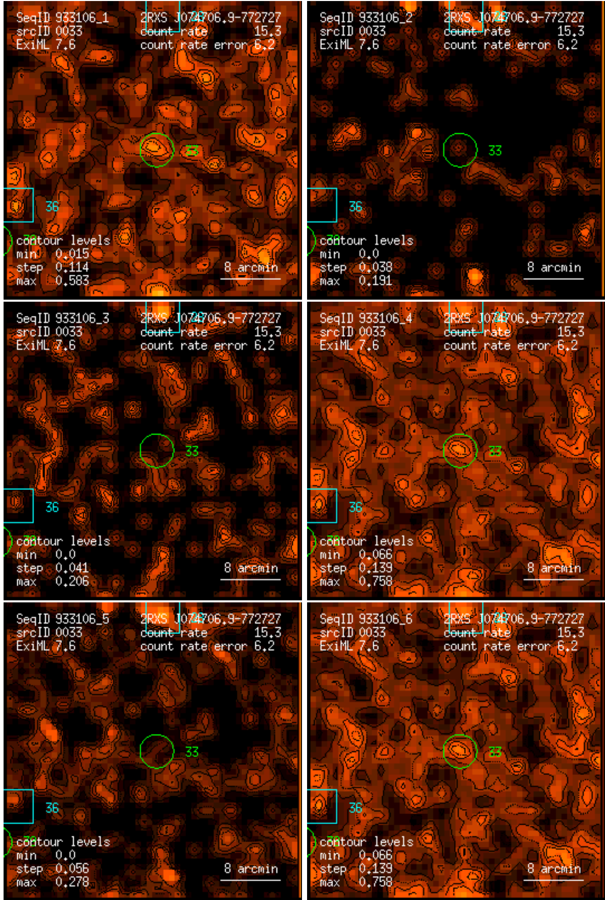
Figure 33: RASS 933106: detection 0033: band rate images, Gaussian filter: (1) PSPC channels 11 – 41, (2) 52 – 90, (3) 91 – 201, (4) 11 – 235, (5) 52 – 201, (6) 11 – 201. Broad band rates in counts/ks. Band rate contour levels in counts/ks/arcmin 2 .
